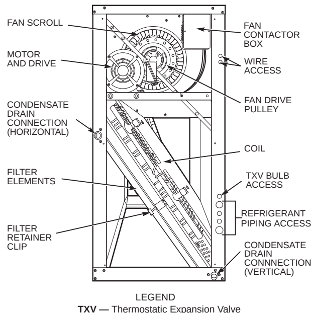
Fig. 15 - Wiring and Service Access (Side Panel Removed)
