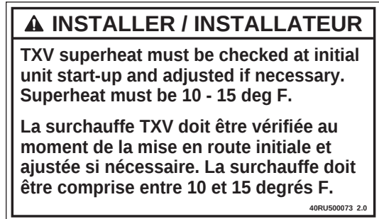
Fig. 21 - Label, TXV Adjustment
