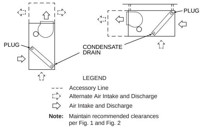
Fig. 5 - Typical Unit Positioning
