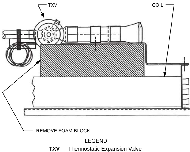
Fig. 4 - Foam Block Location
