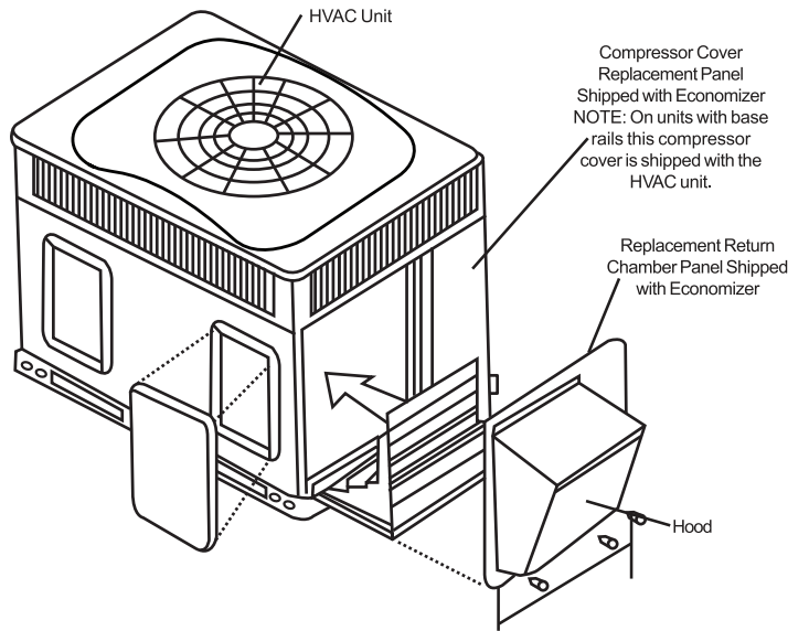
Vertical Economizer
