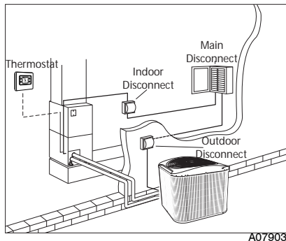
Fig. 1 - Electrical Disconnects
