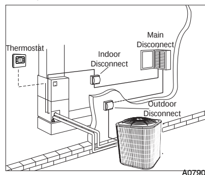
Fig. 1 - Electrical Disconnects
