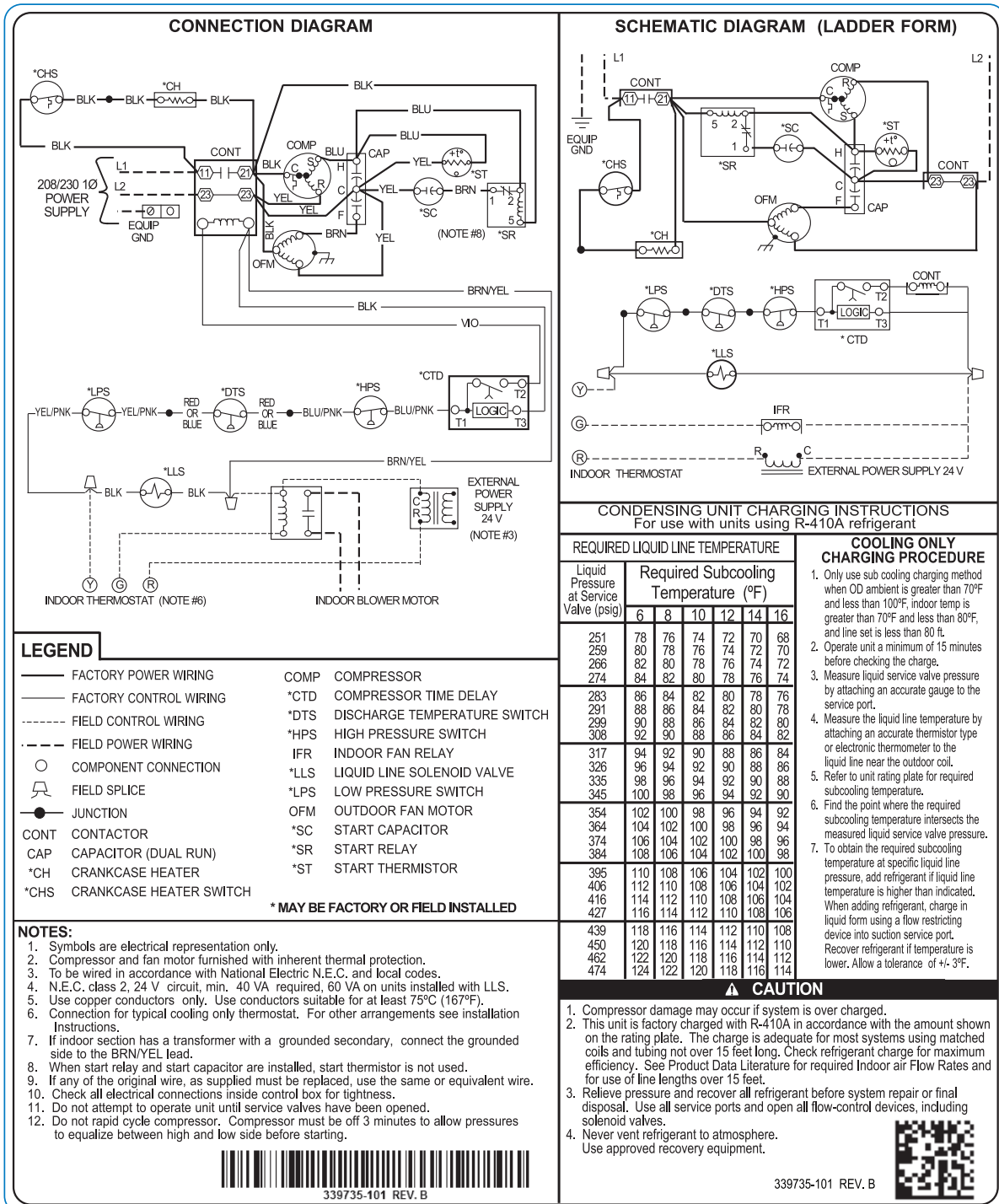
Fig. 1 – Wiring Diagram — Model sizes 1-1/2 - 5 Tons, 208/230-60-1
