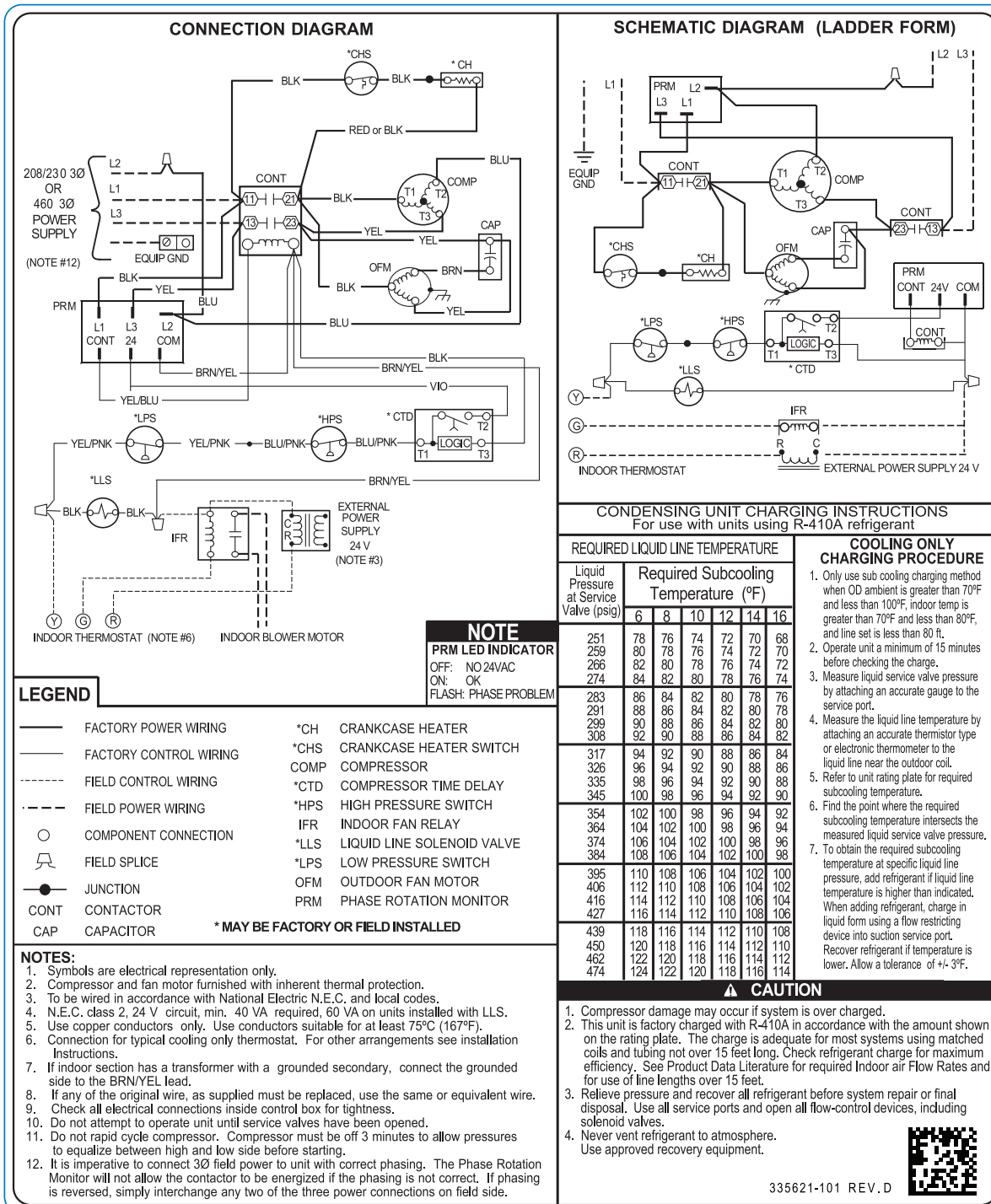
Fig. 1 – Wiring Diagram — Model sizes 3 - 5 Tons, 208/230-60-3
