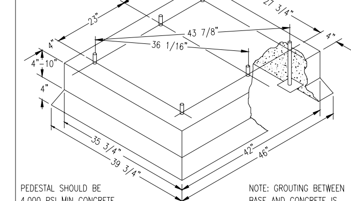
CONCRETE PEDESTAL MOUNTING Figure 1-1
