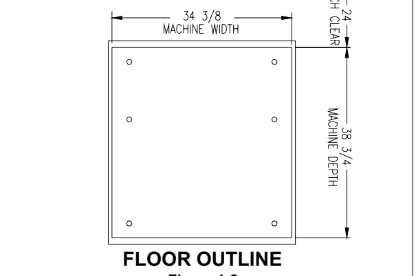
FLOOR OUTLINE Figure 1-2
