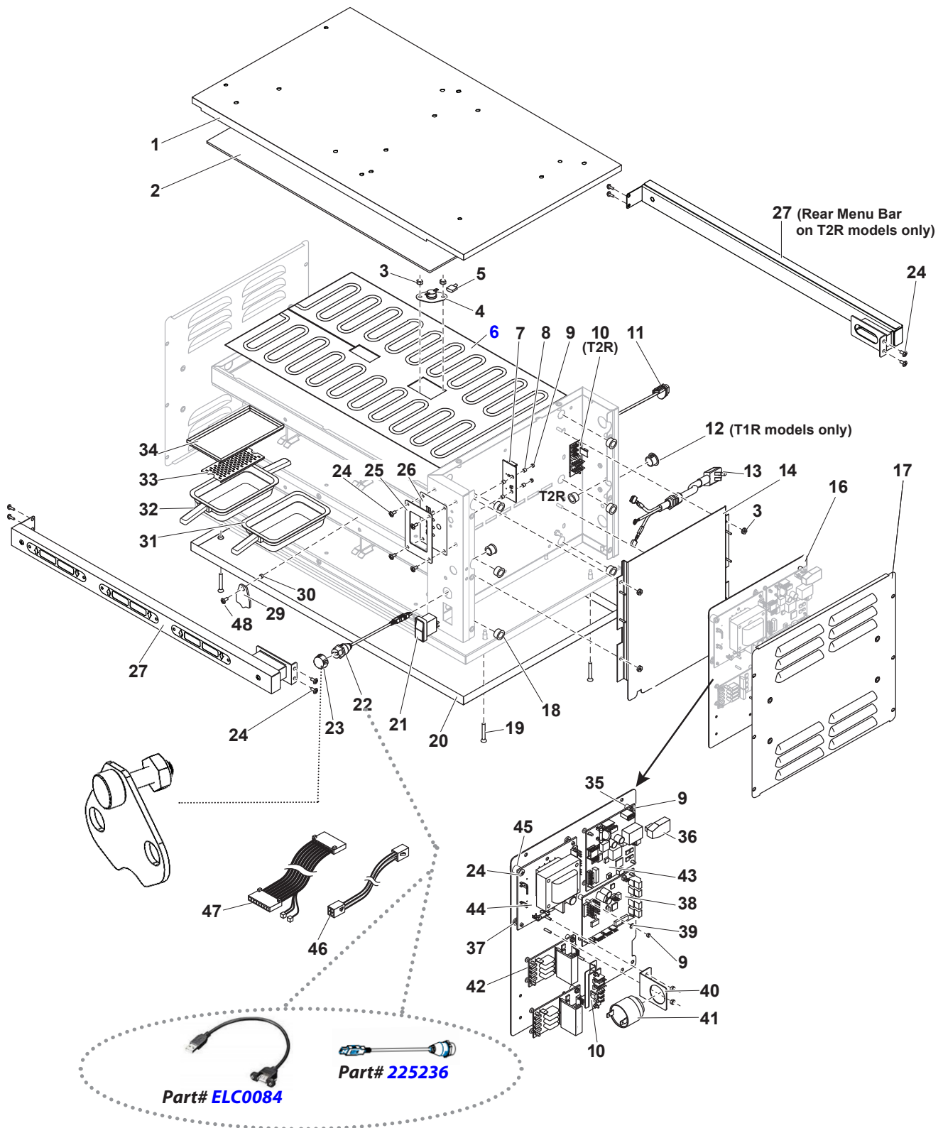
Figure: PL-2 TIMER BAR MODELS HS2-23-1203/1204/2084/2303/2304 T1R, T1P & T2R
