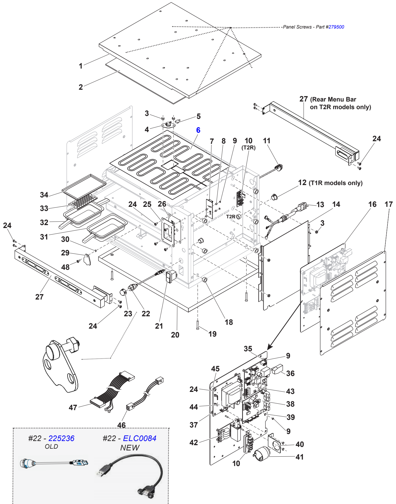
Figure: PL-1 TIMER BAR MODELS HS2-22-2082/2302 T1R & T2R
