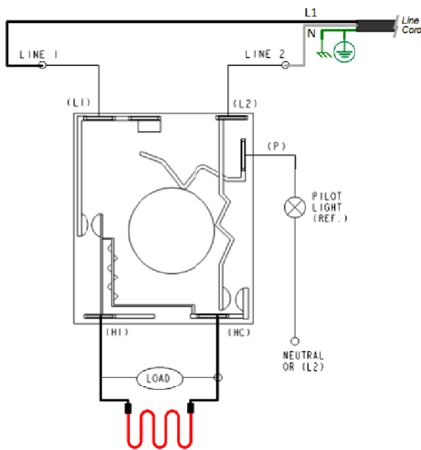
120V Robertshaw
