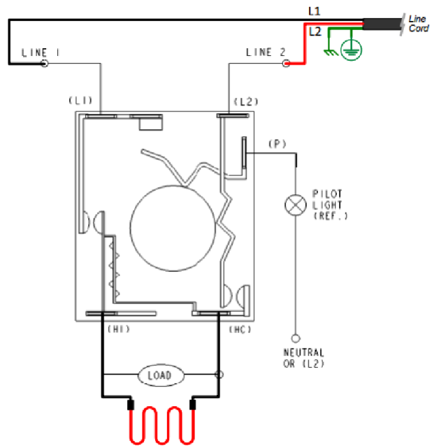
208V/240V Robertshaw
