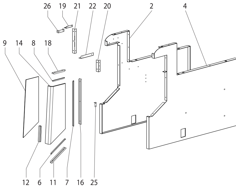
Figure: PL-2 Side Panels
