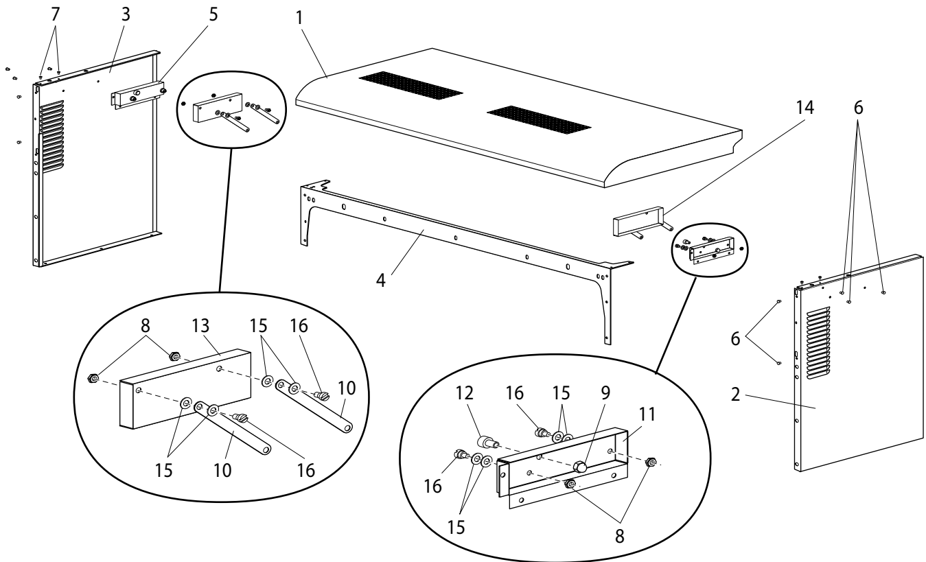
Figure: PL-8 Oven Shield
