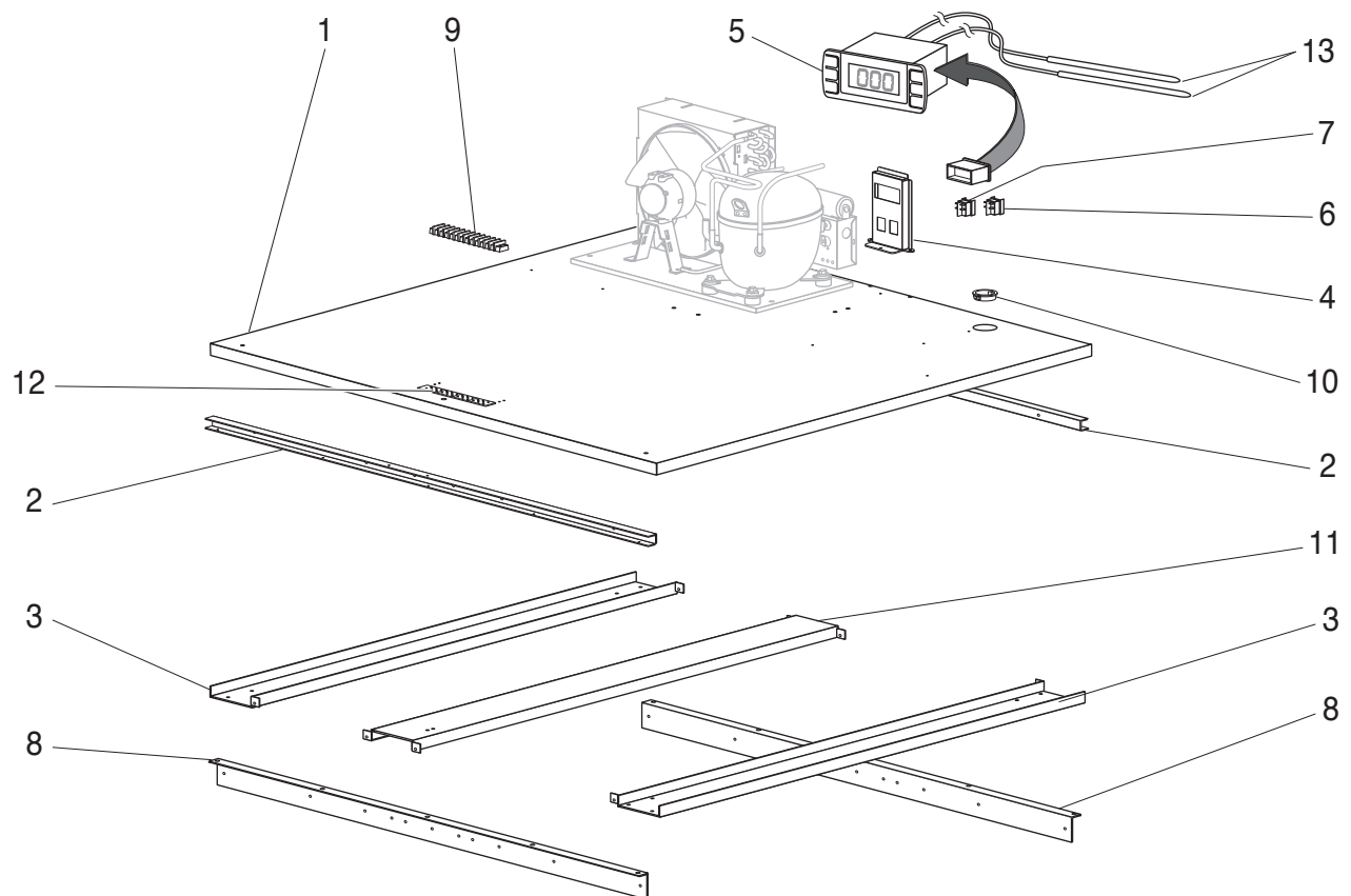
Figure: PL-4 Base Components
