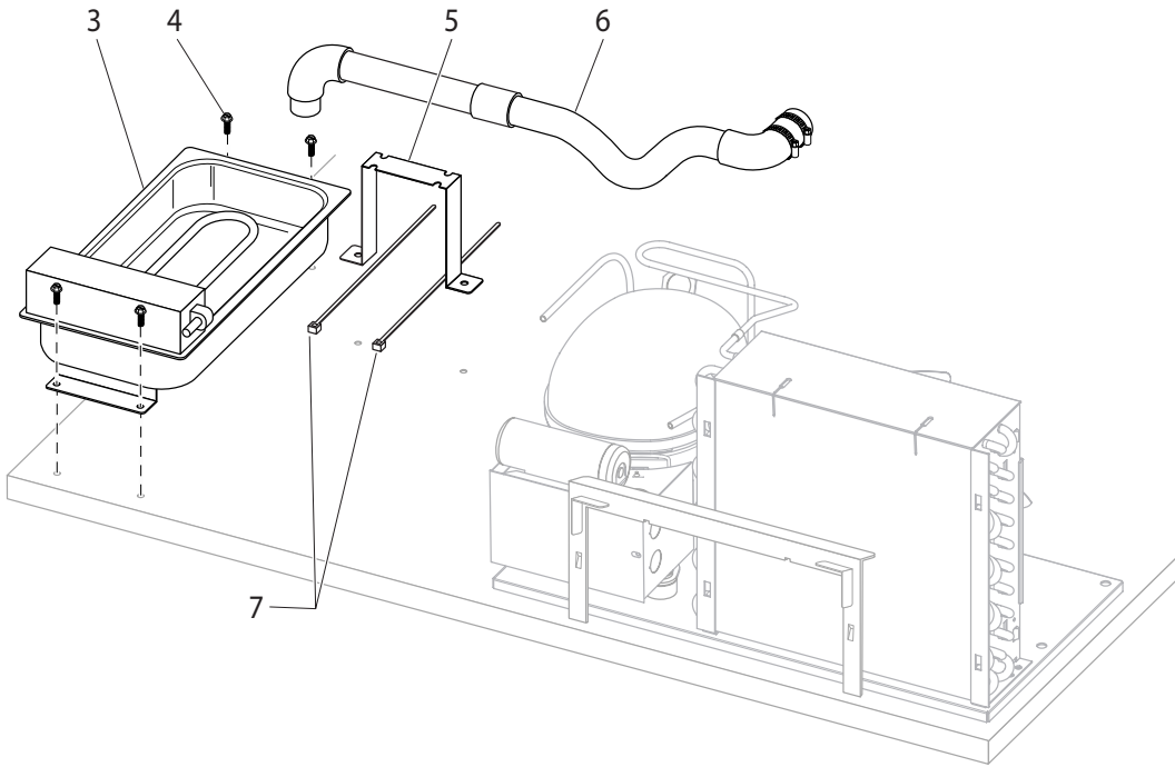
Figure: PL-6 Condenser Compartment Components
