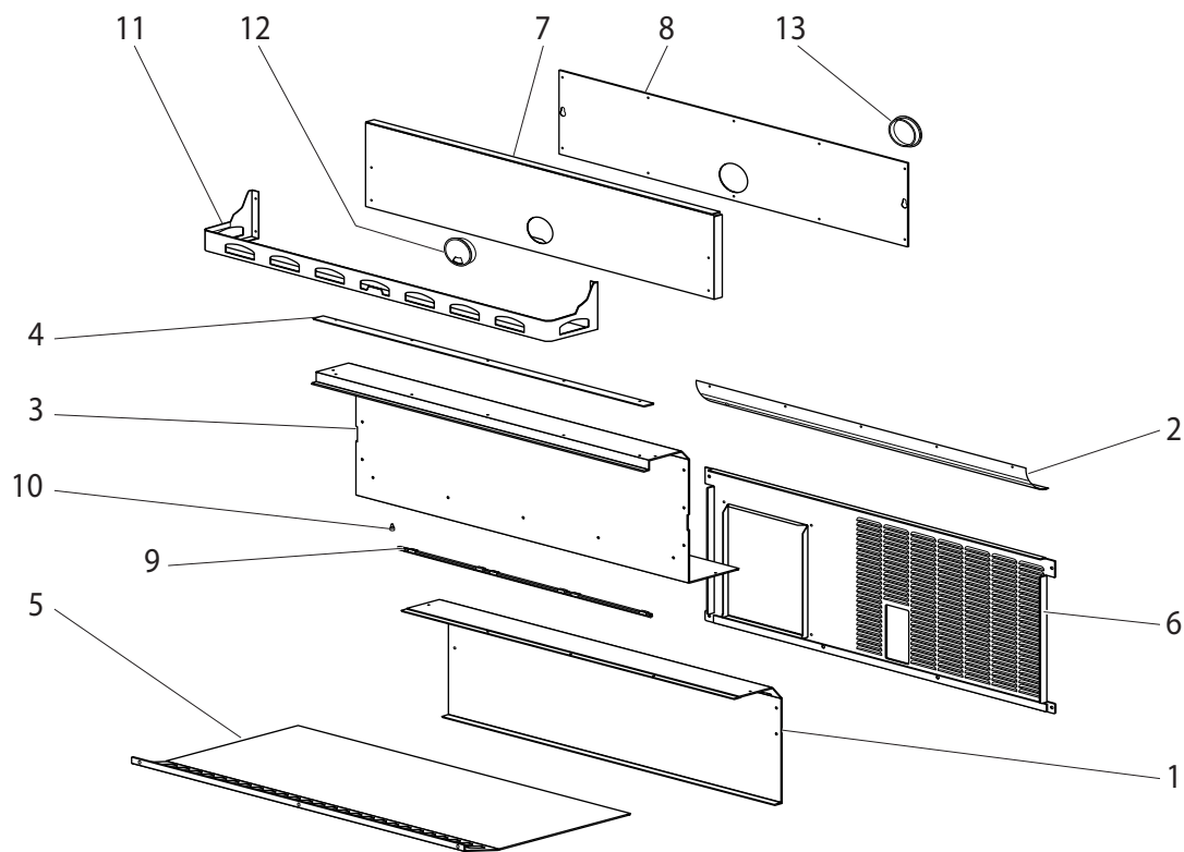
Figure: PL-3 Frame Components
