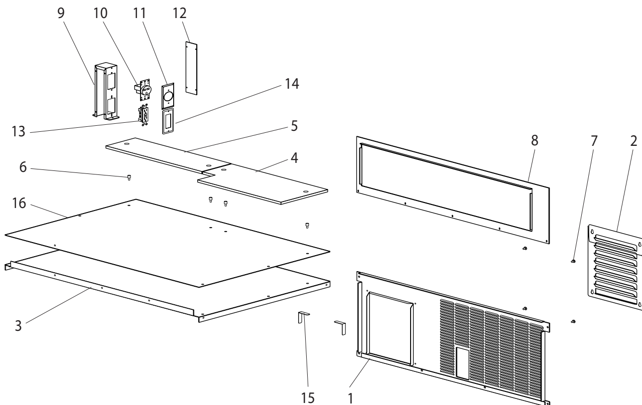
Figure: PL-7 Back Components
