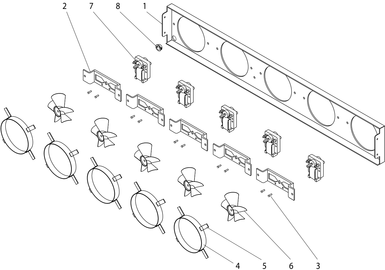
Figure: PL-9 Evaporator Fans Assembly
