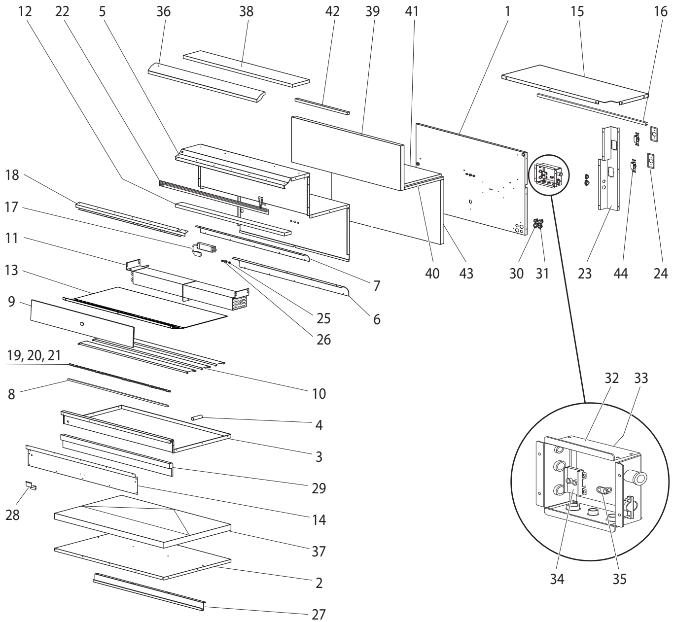
Figure: PL-5 Inside Components
