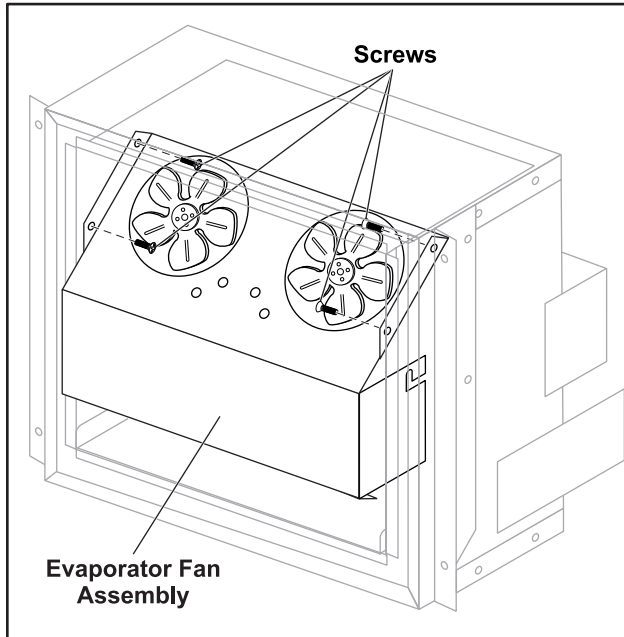
Figure 12. Evaporator Fan assembly
