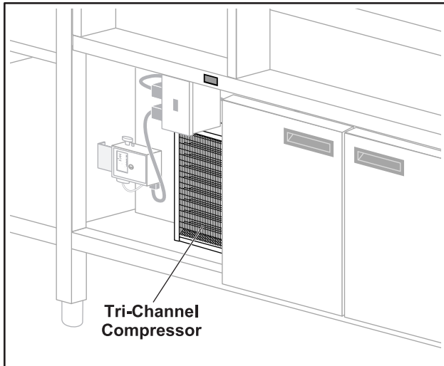
Figure 10. Compressor Assembly
