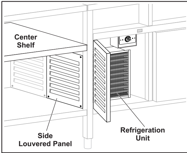
Figure 15. RBC Refrigeration System
