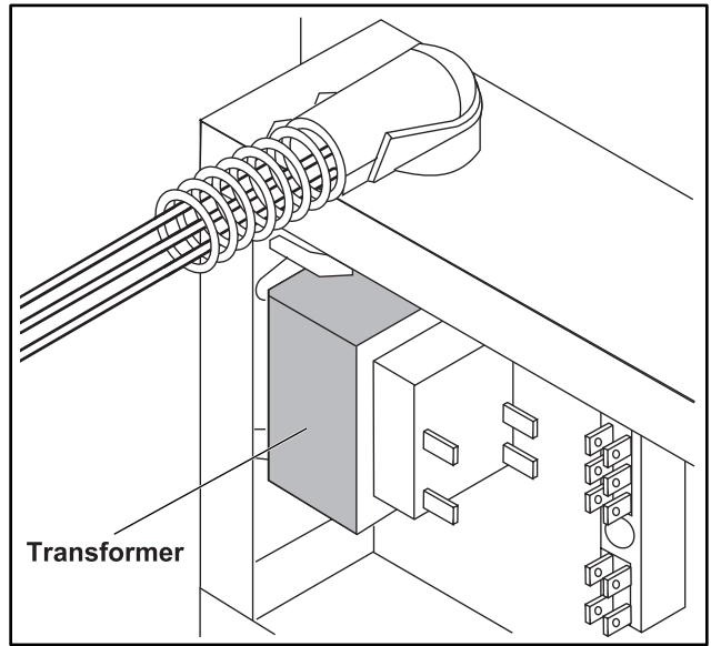
Figure 5. 240/208 Step Down Transformer
