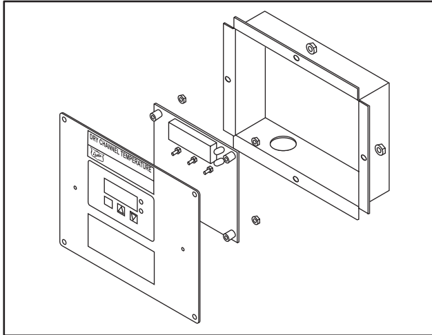
Figure 3. Exploded View of Relay Box Internal Components
