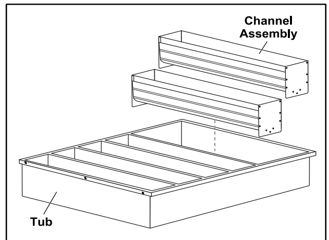
Figure 6. Dry Channel Tub Assembly
