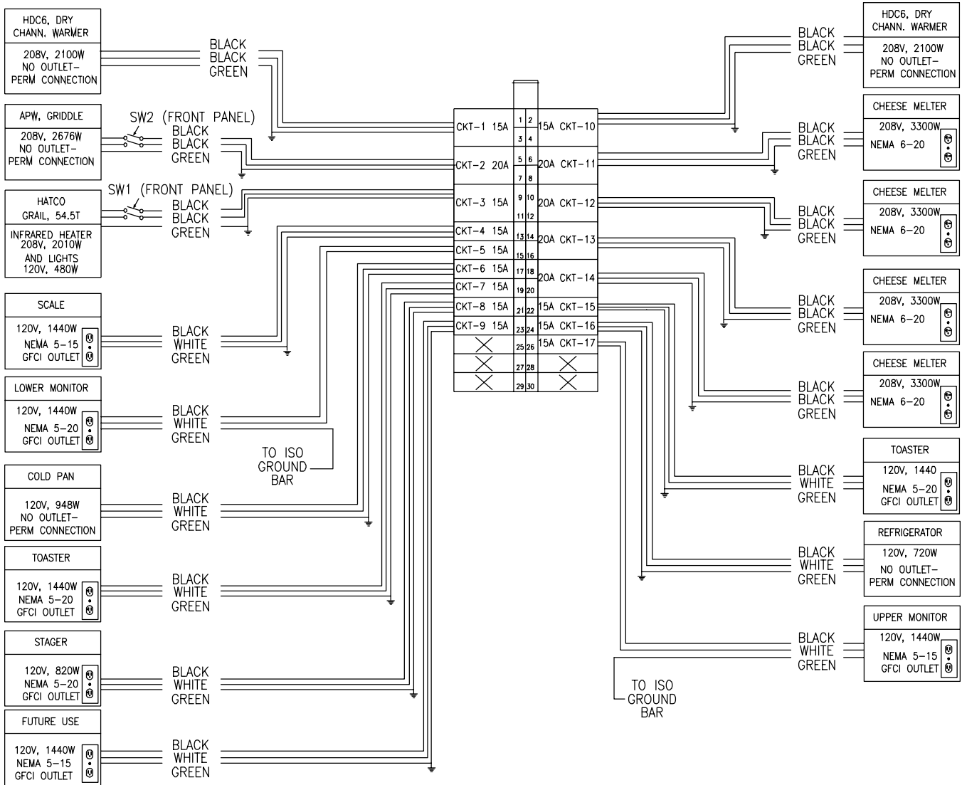
Figure 21. Circuit Diagram
