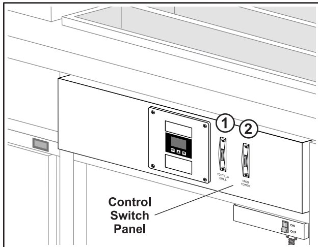
Figure 7. Location of Power ON/OFF switches
