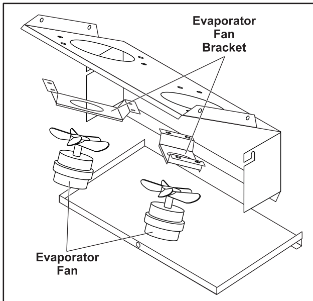
Figure 13. Evaporator Fans
