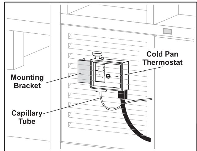
Figure 9. Location of Tri-Channel Cold Pan Thermostat
