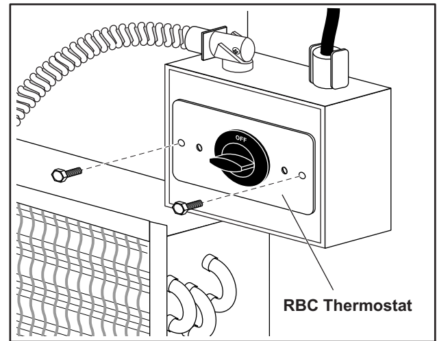
Figure 14. Location of Refrigerator Thermostat
