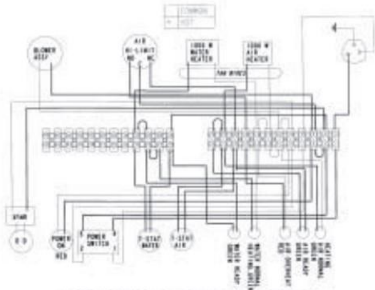
WIRE DIAGRAM FOR PROOFER ONLY MODULE
