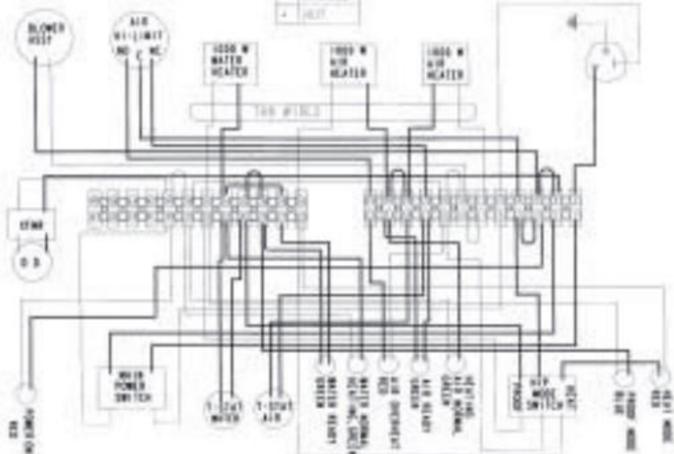
WIRE DIAGRAM FOR HEATED/PROOFER MODULE
