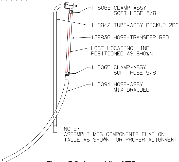
Figure 7-6 Assembling MTS
