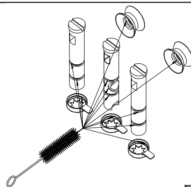
Figure 6-7 Clean O-ring grooves, seal and nozzle with brush.
