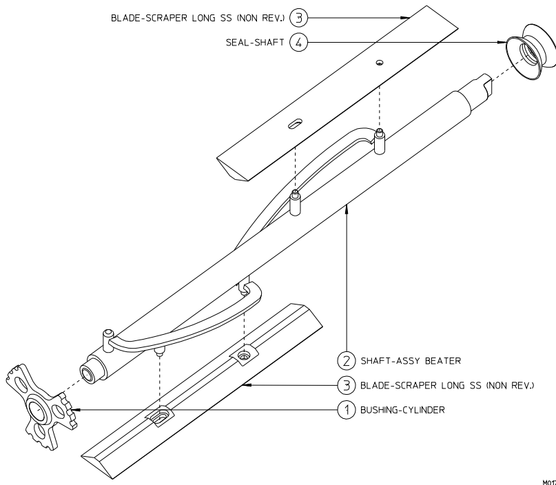
Figure 6-3 Beater Shaft Assembly
