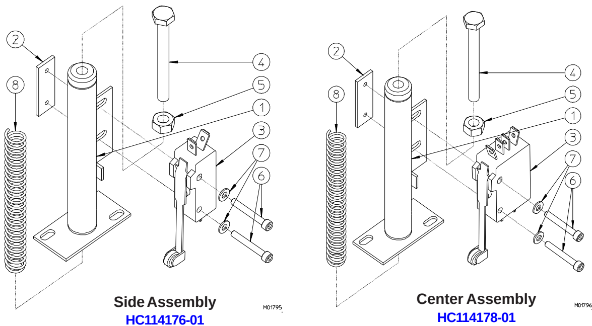
Figure 6 Switch Assemblies
