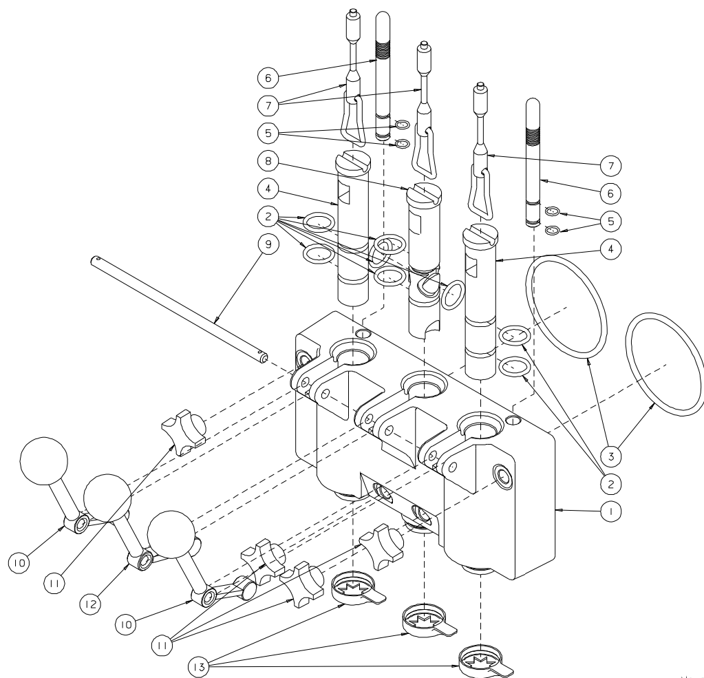
Figure 1 Head Assembly
