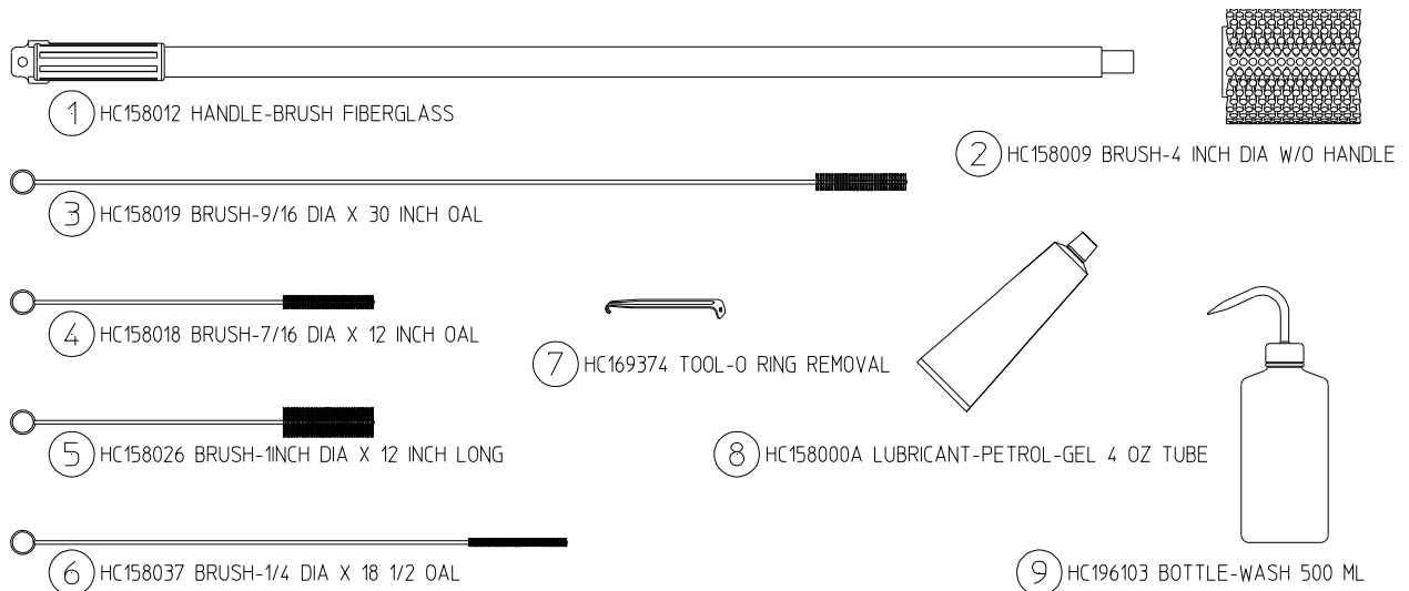
Figure 6-1 Cleaning Accessories
