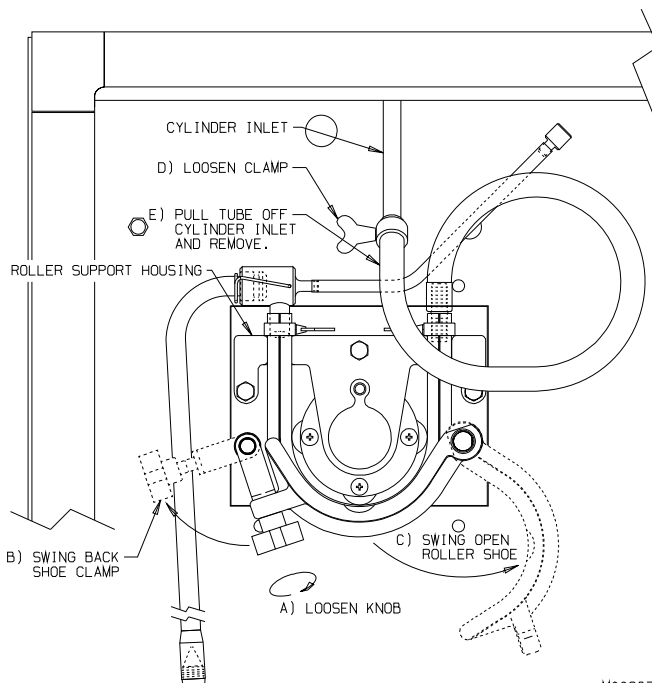
Figure 6-4 MTS
