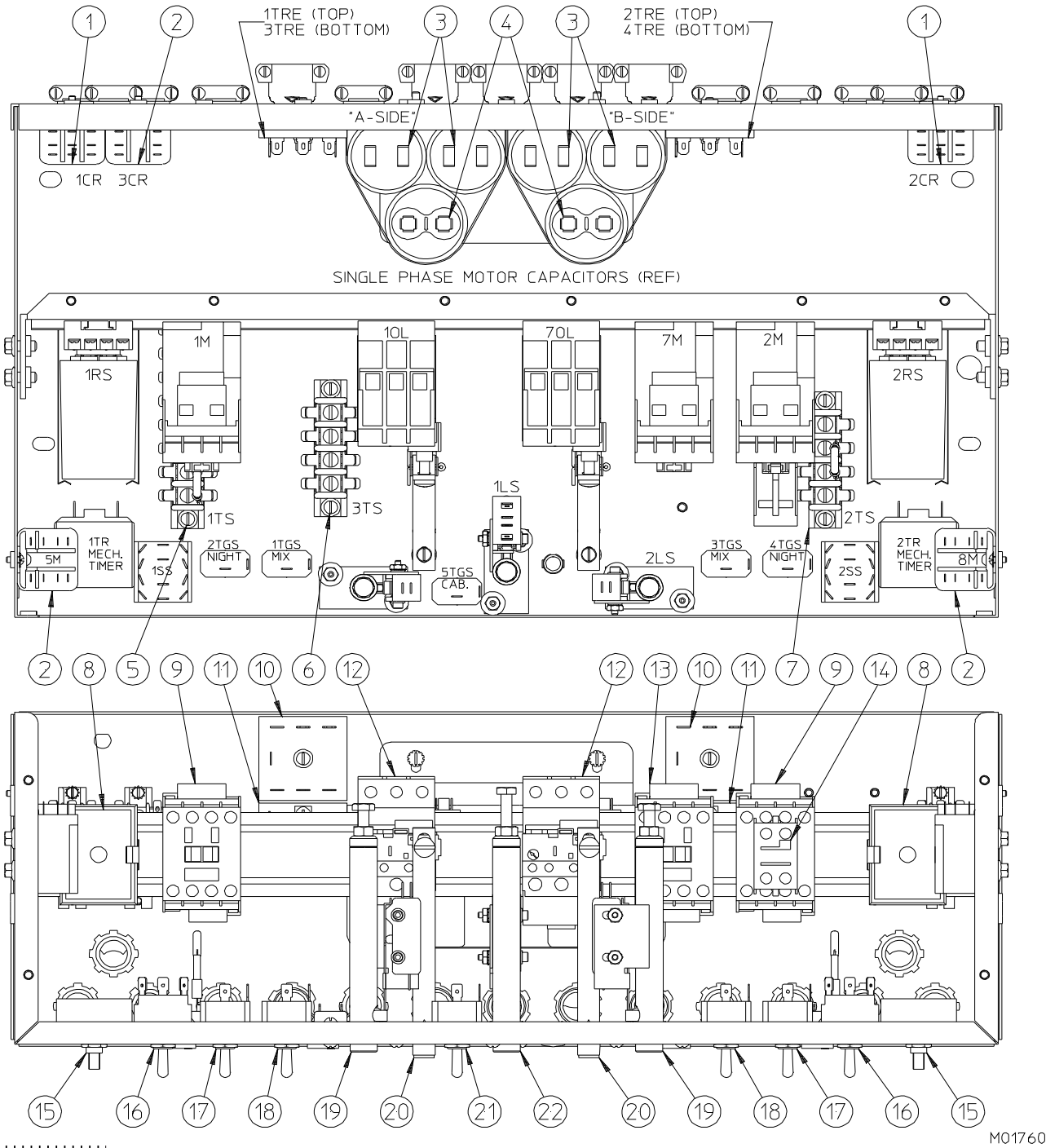
Figure 7 Switch Box (sheet 1 of 2)
