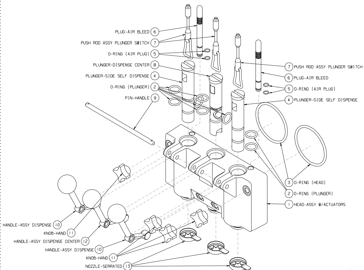
Figure 6-2 Head Assembly
