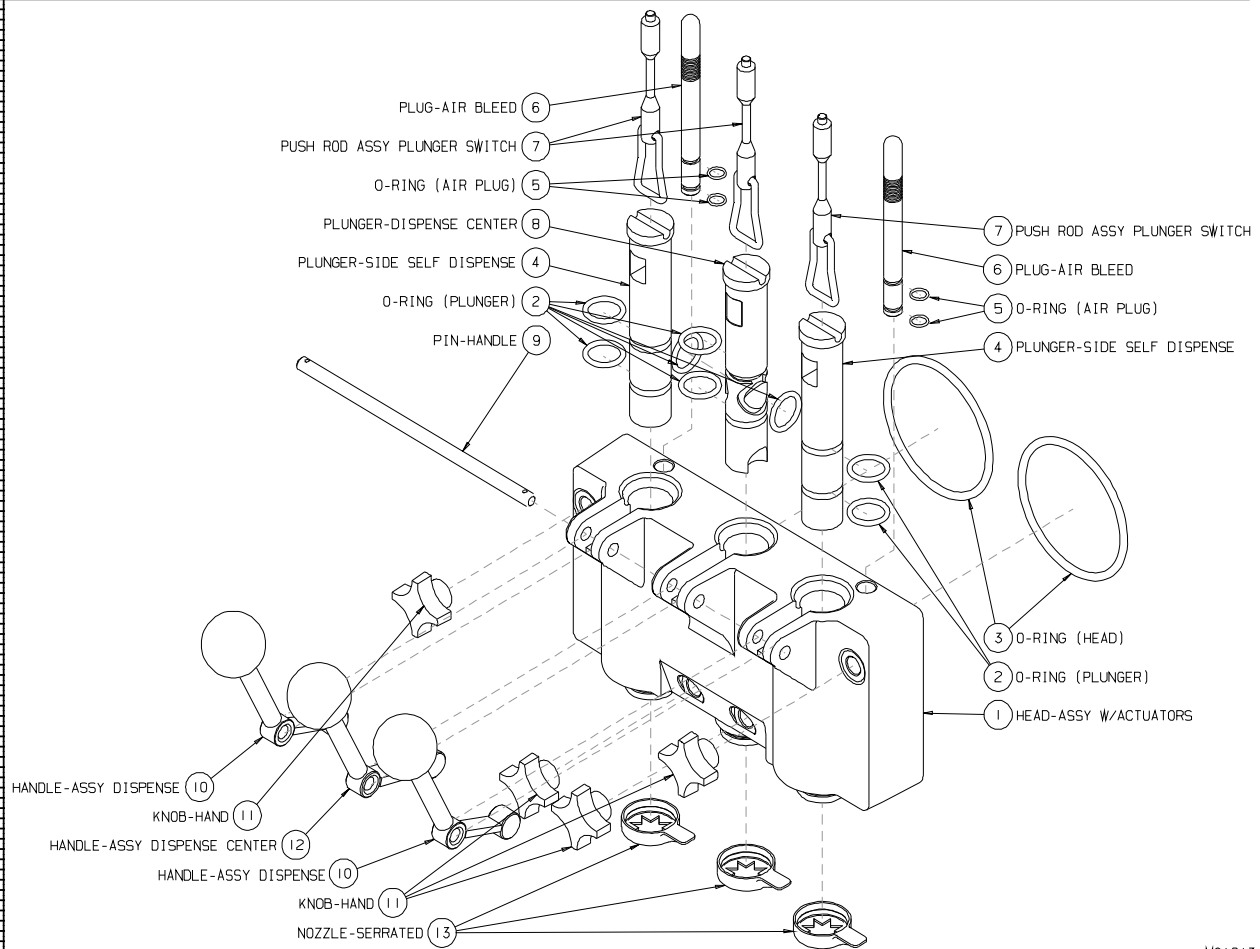
Figure 7-4 Dispense Head Assembly
