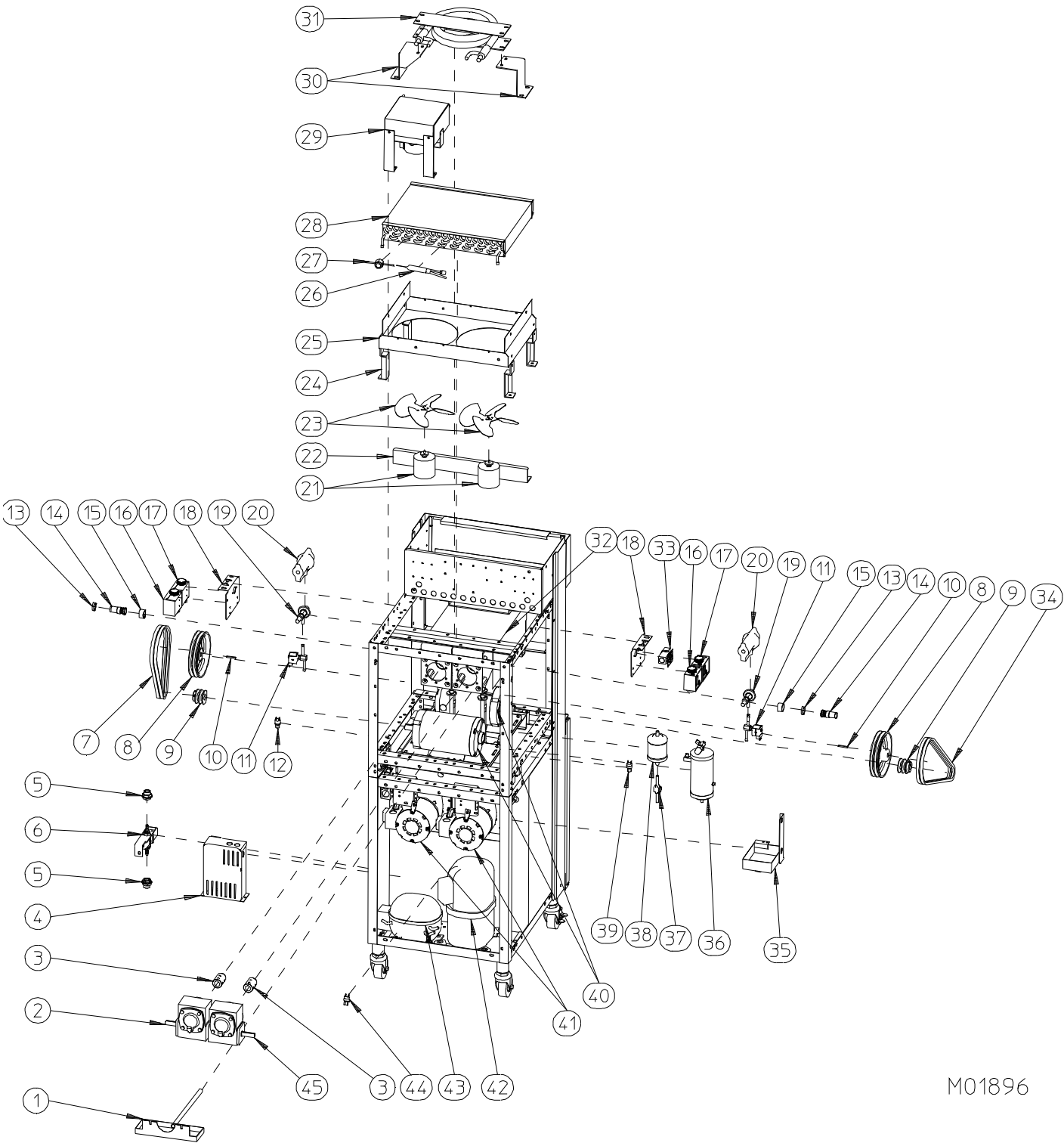
Figure 9 Assembly Views (sheet 1 of 2)
