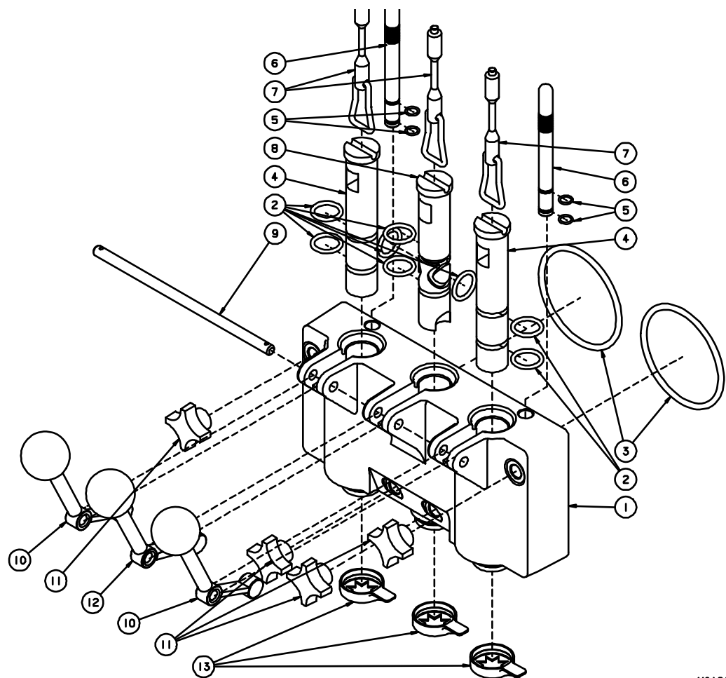
Figure 1 Head Assembly
