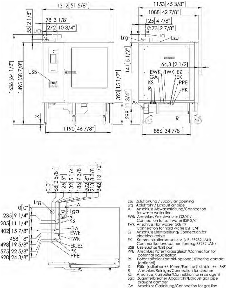
Fig. 29: GeniusMT 12-21, gas, right-hinged
