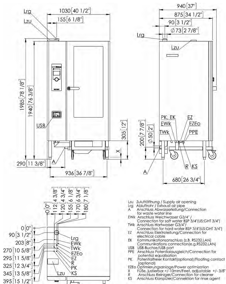
Fig. 25: Multimax 20-11, electric, right-hinged
