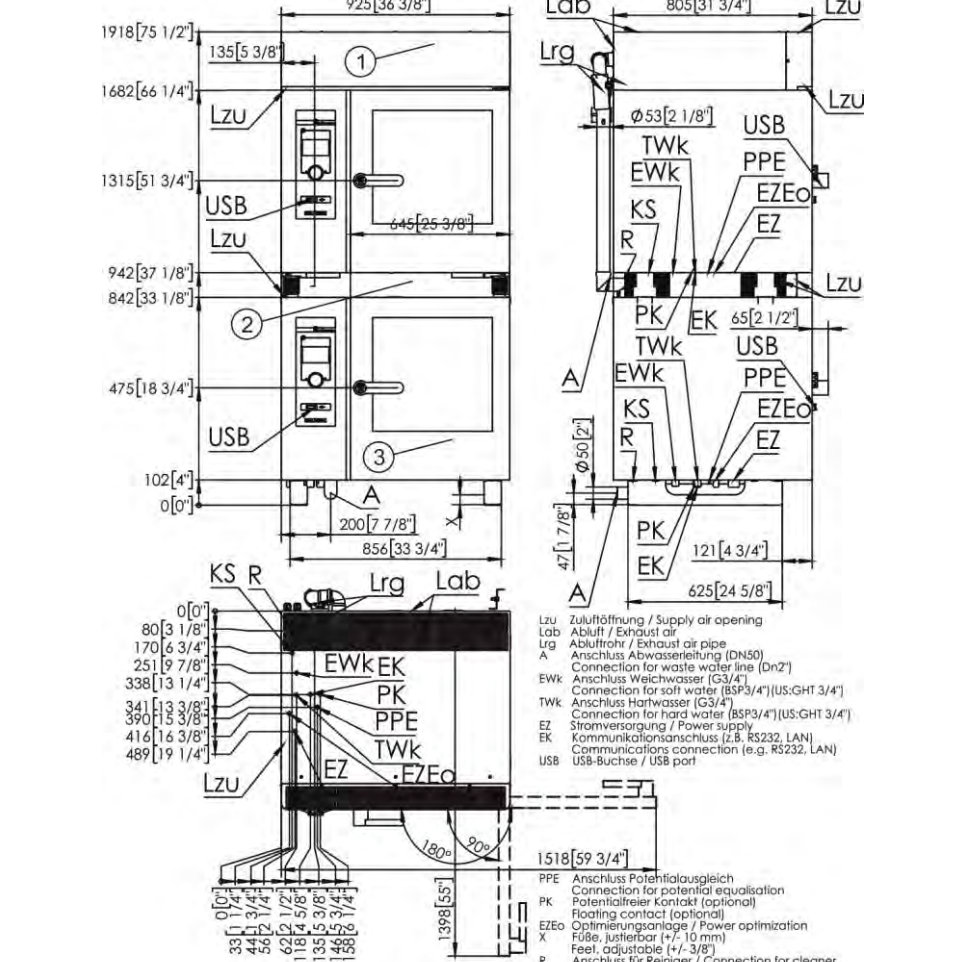
Fig. 34: Kombimix station sizes 6-11/6-11 with condensation hood KH2, right-hinged
