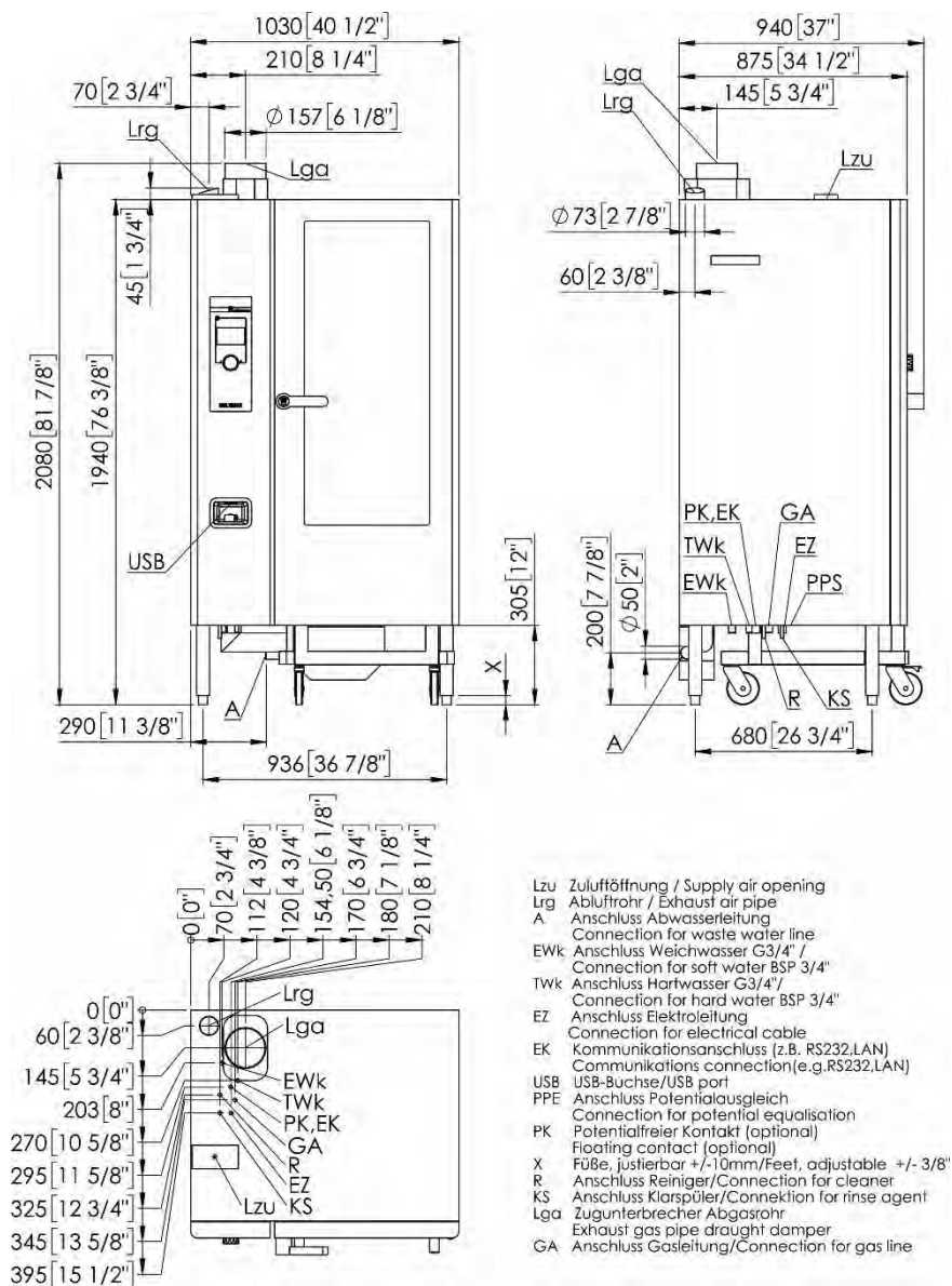
Fig. 27: Multimax 20-11, gas, right-hinged
