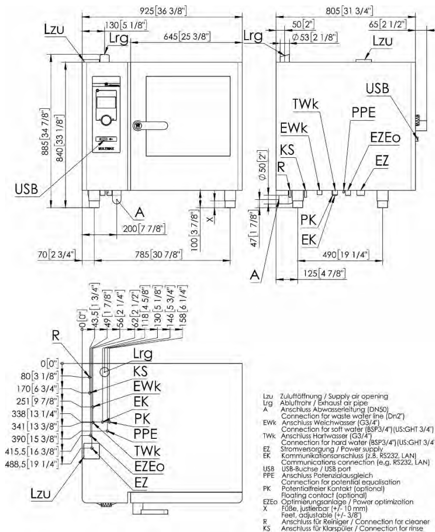
Fig. 14: Multimax 6-11, electric, right-hinged
