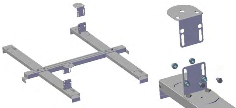
Fig. 50: Foot mounts
