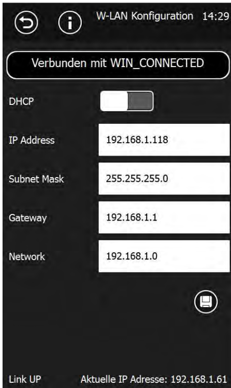
Fig. 11: WLAN configuration
