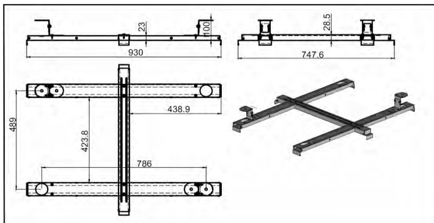
Fig. 45: Intermediate frame installed (Kombimix kit, right-hinged 6-11/10-11 ELECTRIC)
