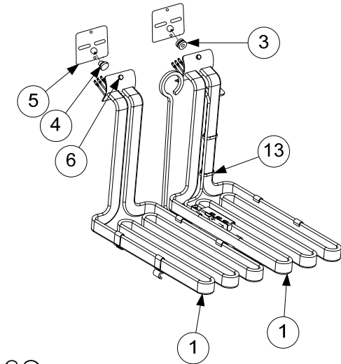
FULL-VAT ELEMENT ASSEMBLY
