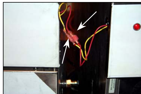
Figure 3. Yellow and red wires connecting oil return switches.
