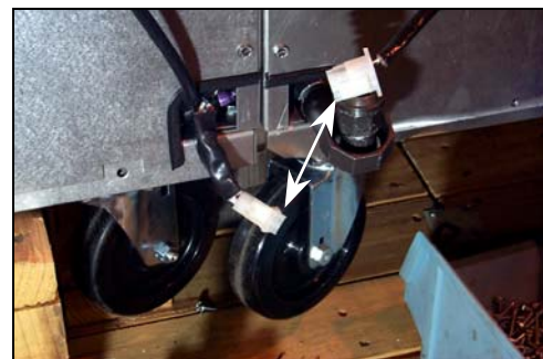
Figure 5. Connect oil-return line heater-tape connectors.
