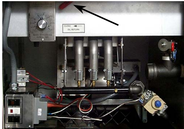
LJS 24G oil-return handle location.
