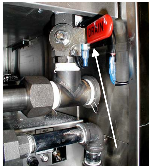
LJS 24G drain valve location.
