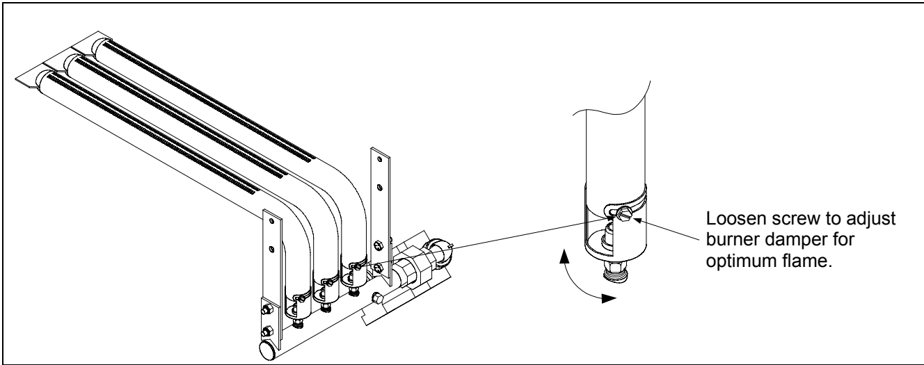
Figure 2: Burner damper adjustment on burner tubes.
