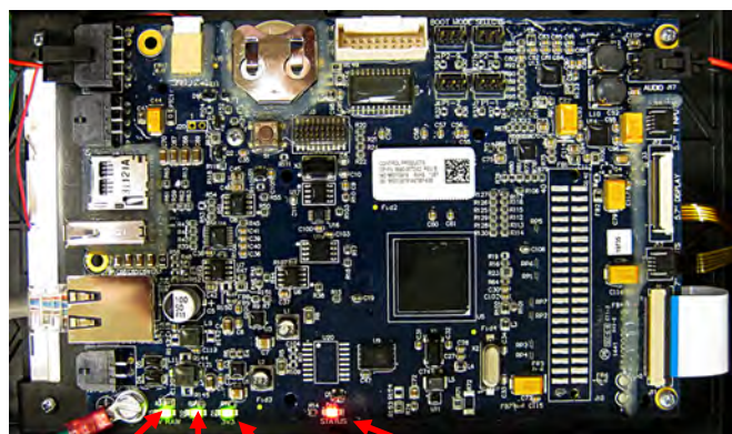
12V from SIB 5V from SIB 3V from power supply on UIB When the touch screen is pressed the STATUS LED illuminates RED.
