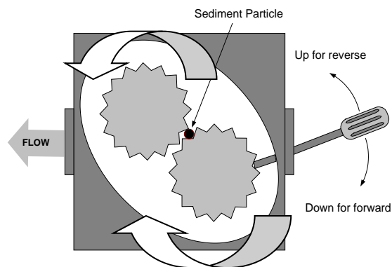
Figure 37 Internal Oil Flow is illustrated by large arrows.
