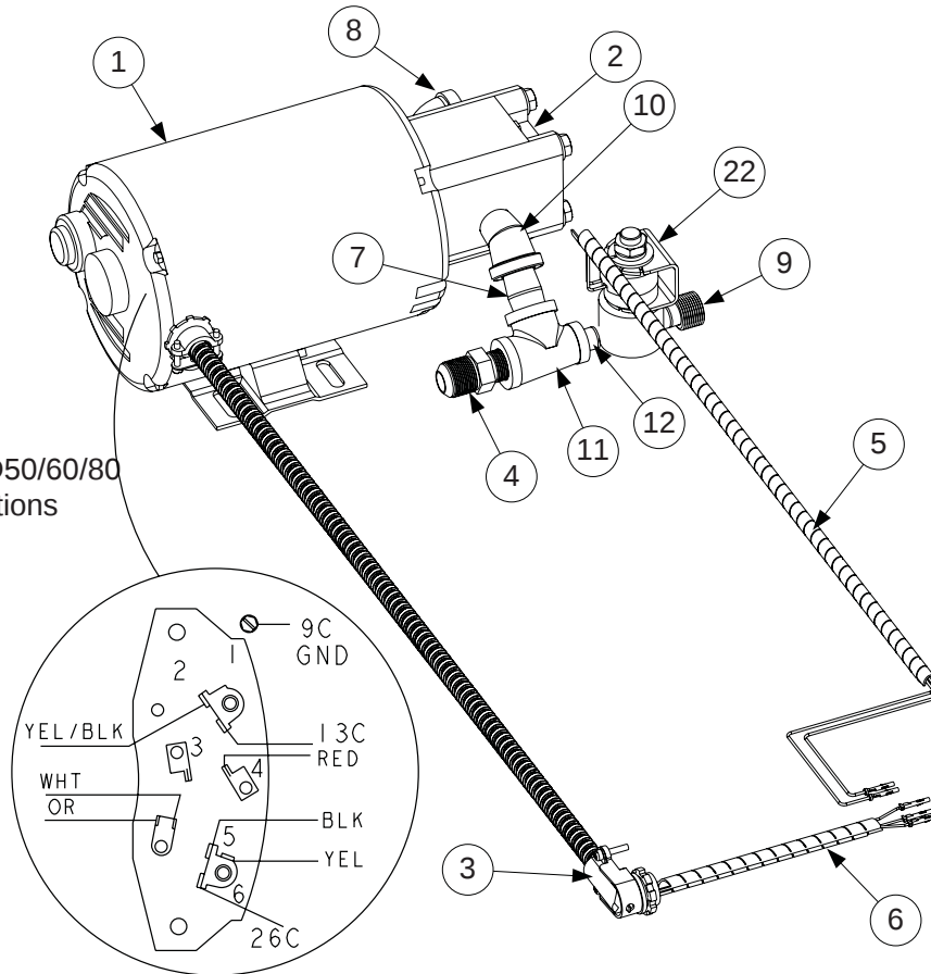
Filter Pump Wiring
