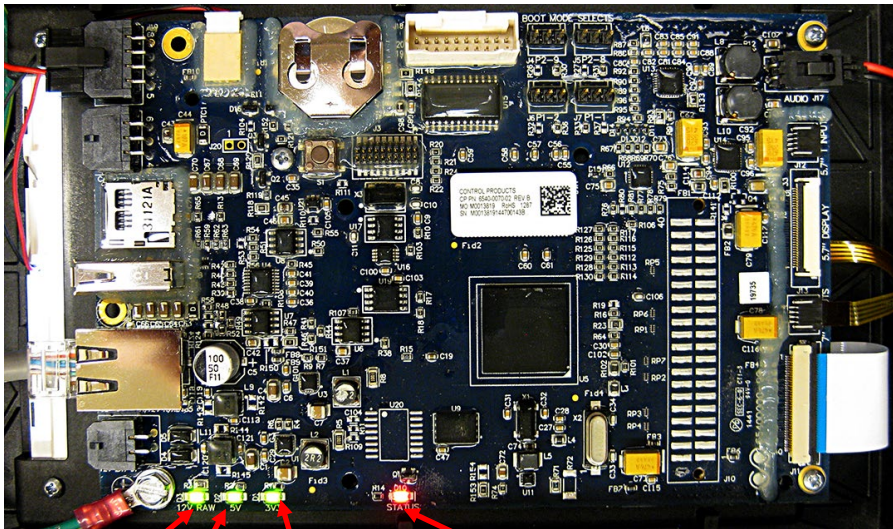
Figure 7 12V from SIB 5V from SIB 3V from power supply on UIB When the touch screen is pressed, the STATUS LED illuminates RED.
