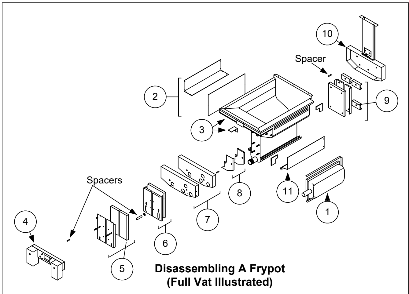
Figure 20 See page 1-26 for reassembly illustration.
