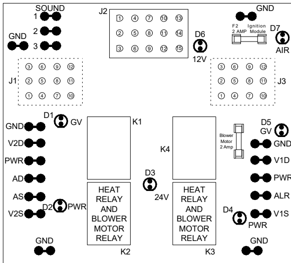
INTERFACE BOARD P/N 106-0386SP
