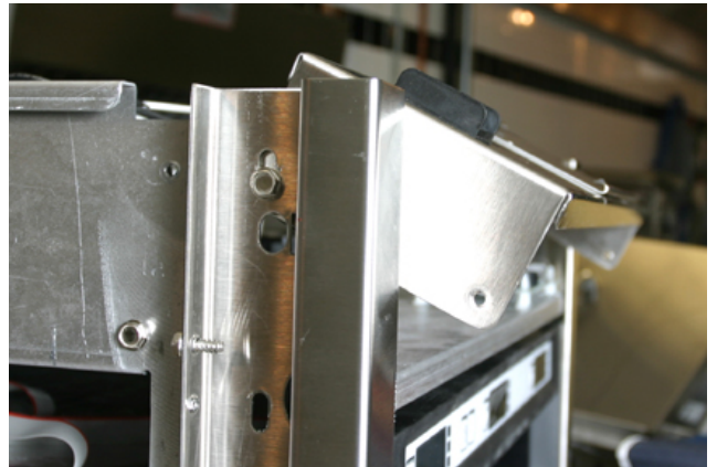
Figure 3: Remove the screws which secure the component shelf, allowing the shelf to be pulled forward.
