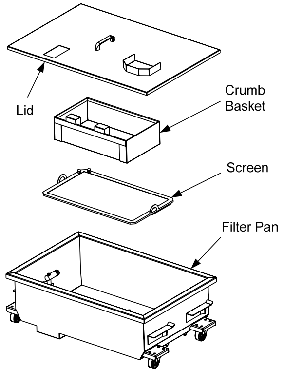
Filter pan assembly.
