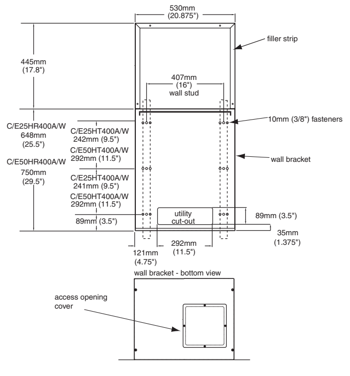
Fig. 8 – Mounting dimensions with wall mount units without drain pan with integral ice machine
