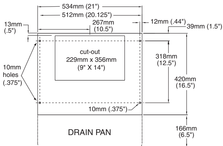
Fig. 2 – Counter cut-out, all models
