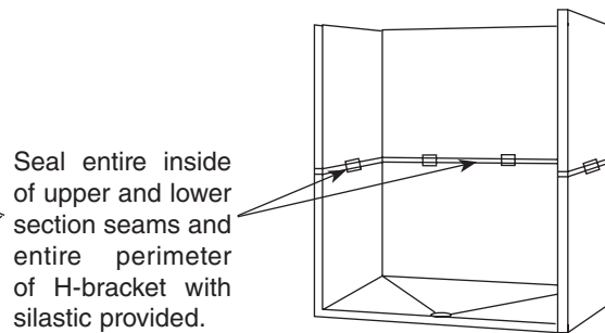
Fig. 3 – Bin Cutaway
