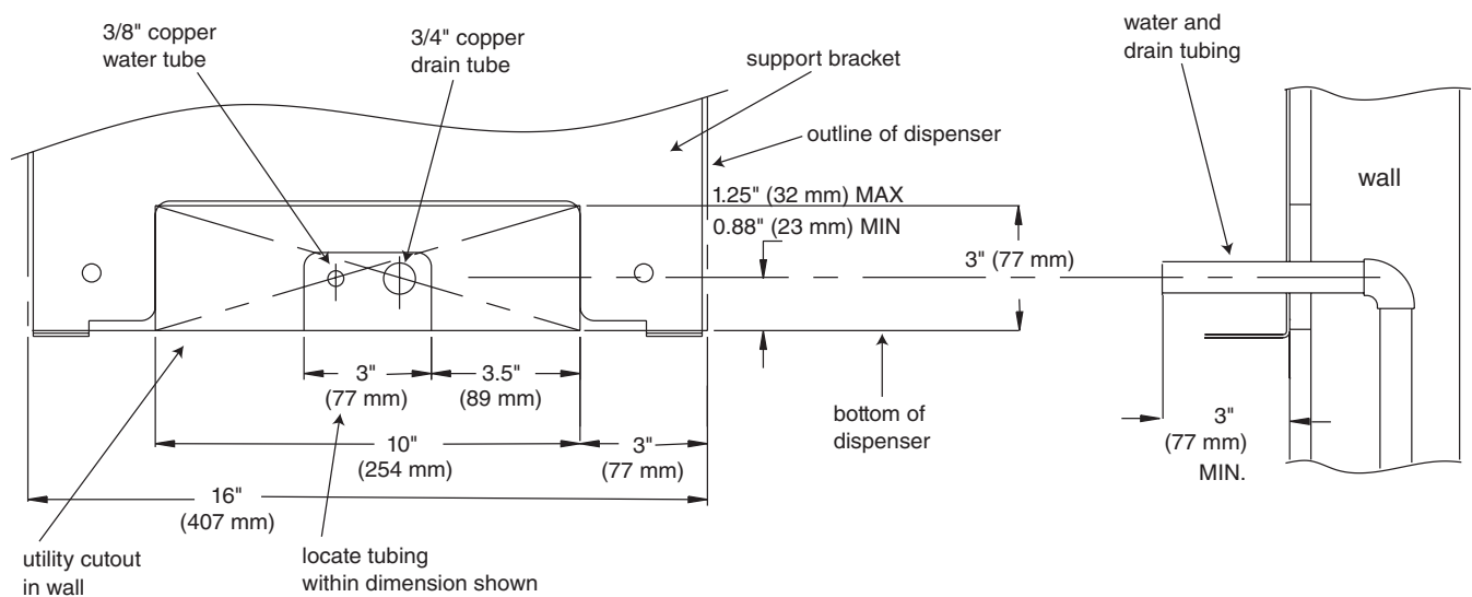
Side view of utilities exiting wall
