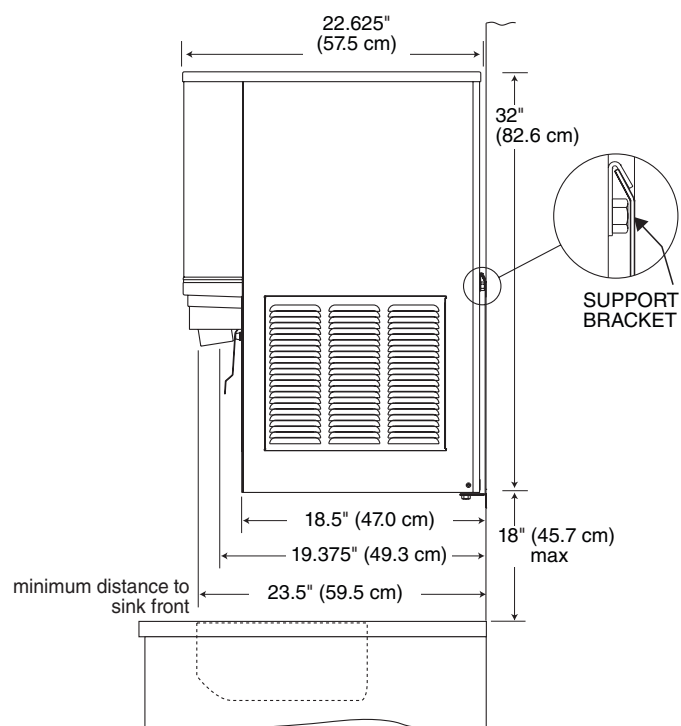
Fig. 7 – Wall mount side view
