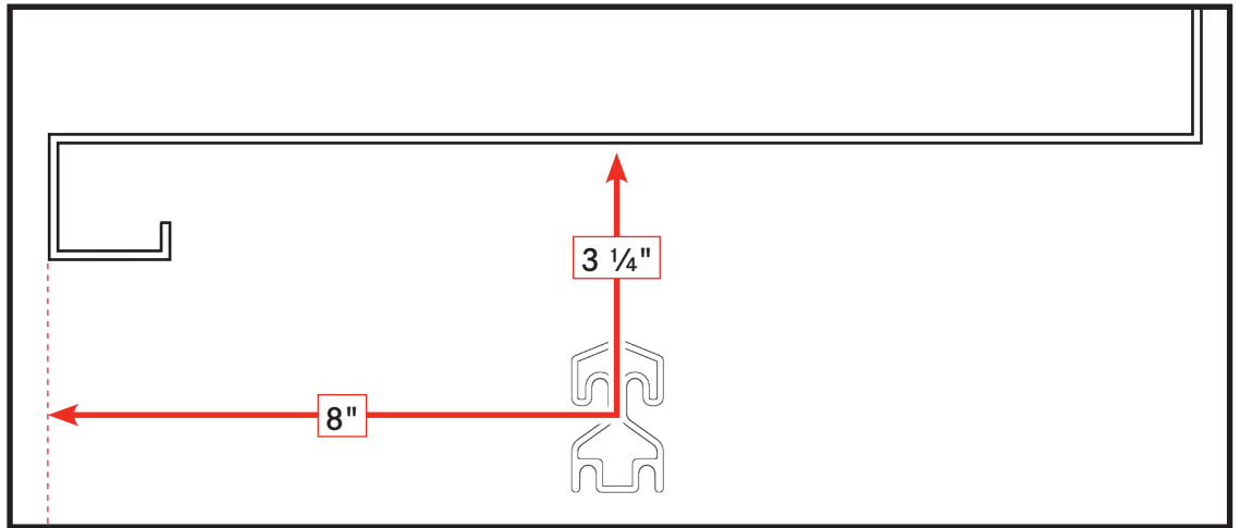
DETAIL B
