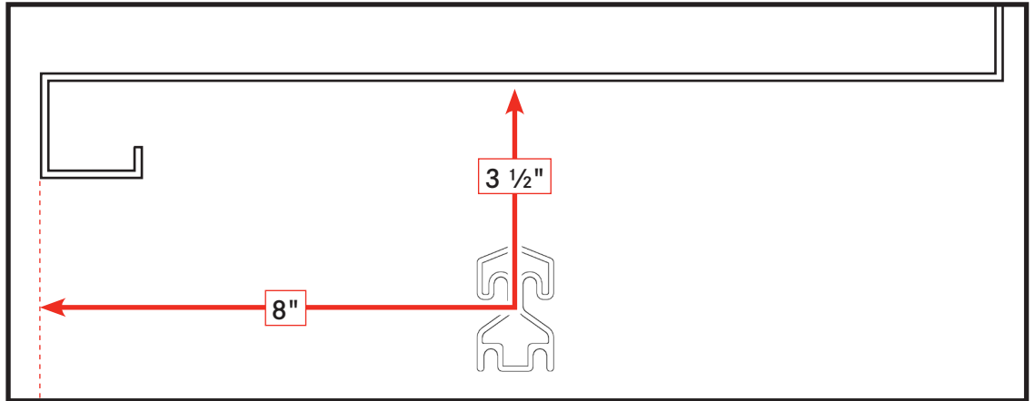
DETAIL G
