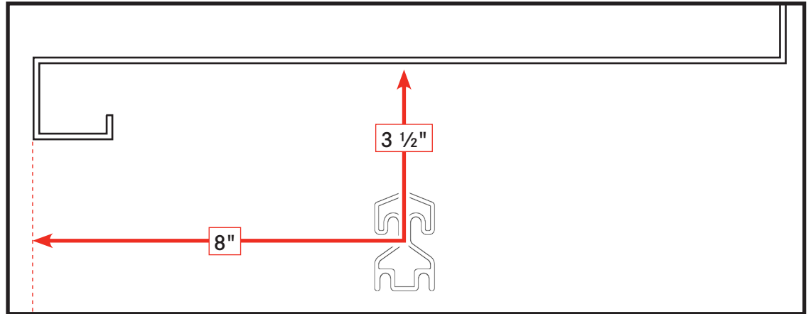
DETAIL D
