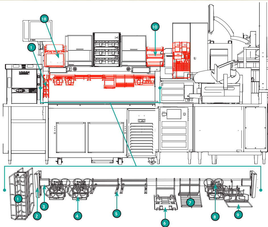
Item# 27807957 Rev. B System, dual line (main)
