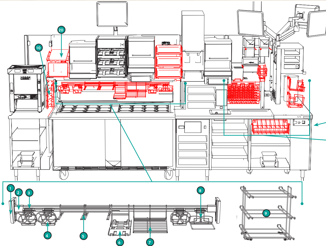
Item# 27807958 Rev. B System, linear line (main)
