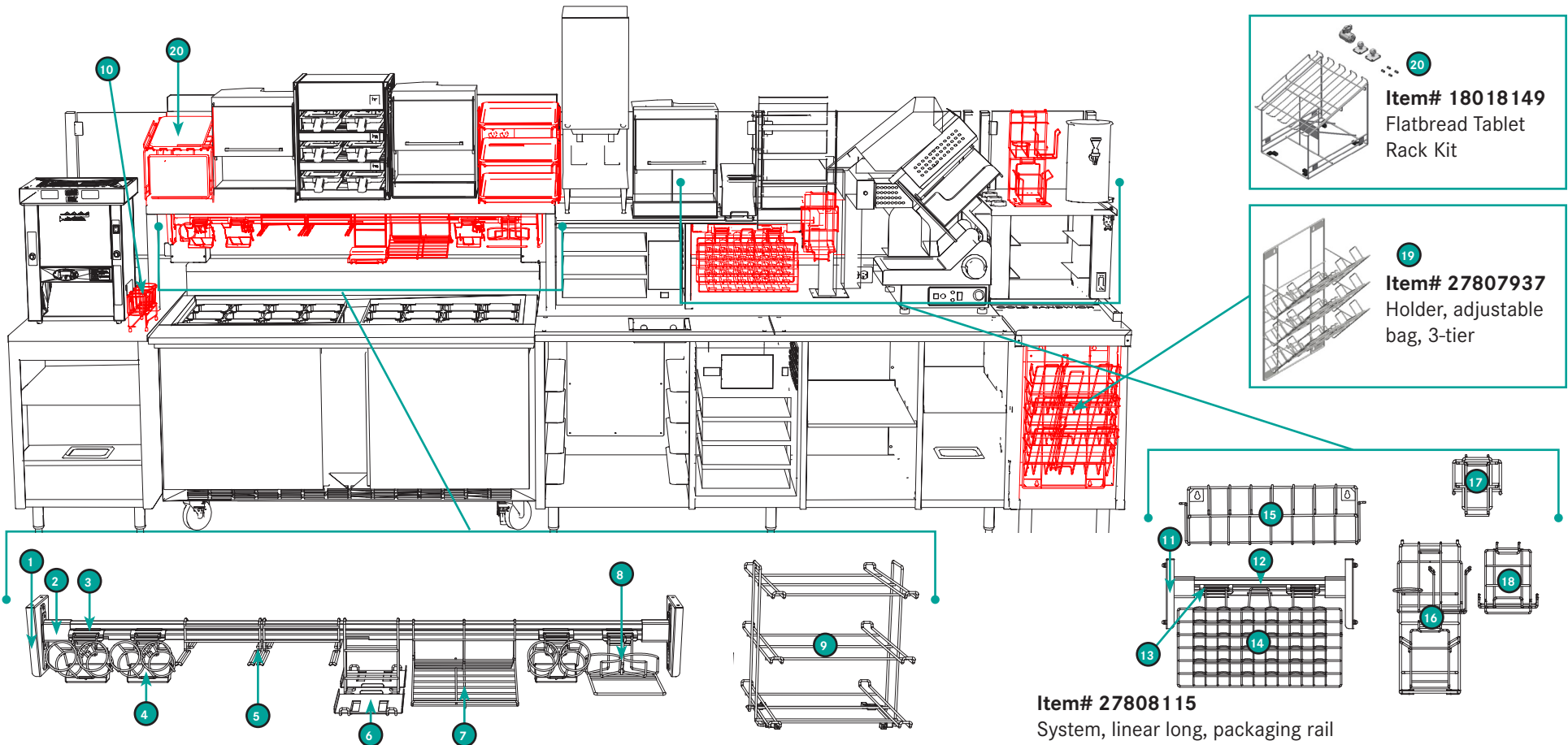
Item# 27807958 Rev. B System, linear line (main)
