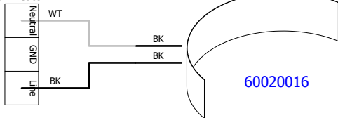
J2 Heater
