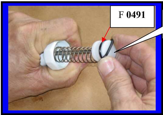
Installing Plunger Assembly into Faucet body
