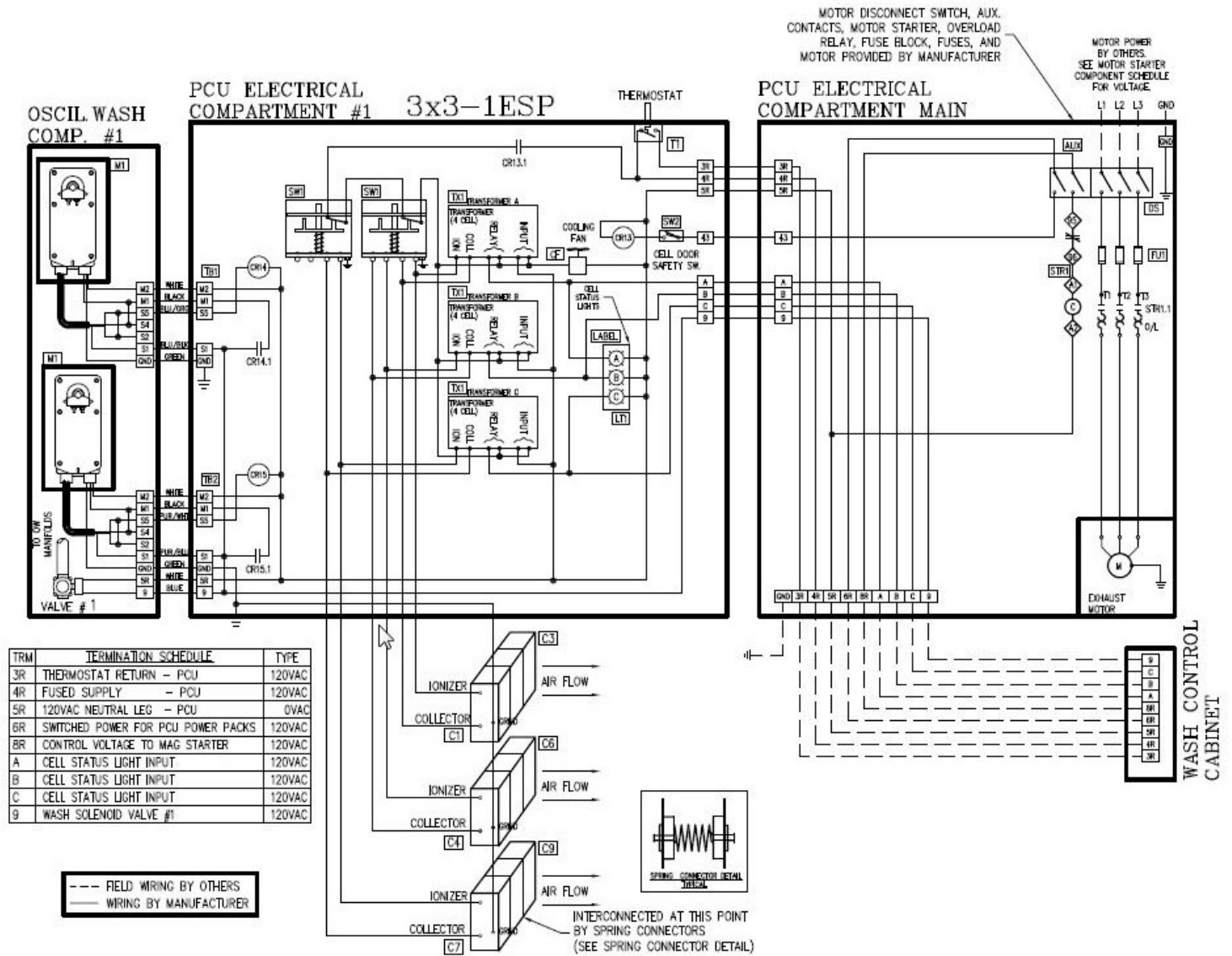
Figure 8-3-1 Wiring For 3x3-1ESP
