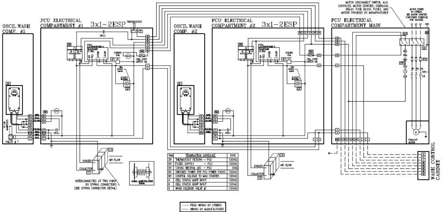
Figure 8-6-1 Wiring For 3x1-2ESP
