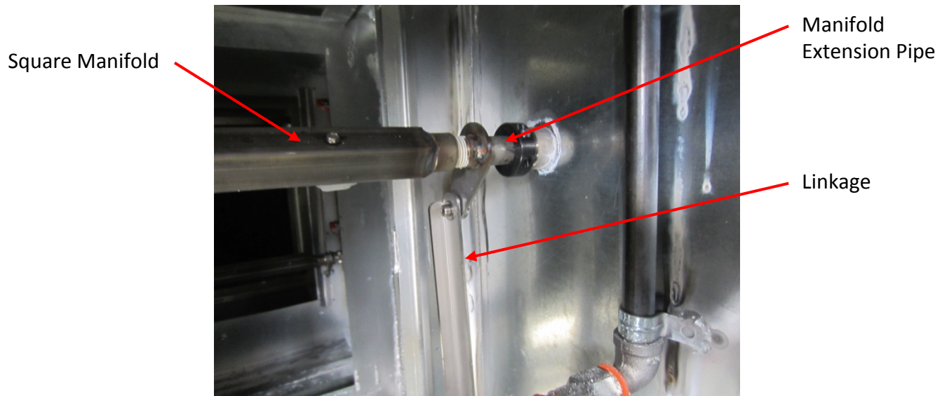
Figure 4-36-1 Motor Manifold
