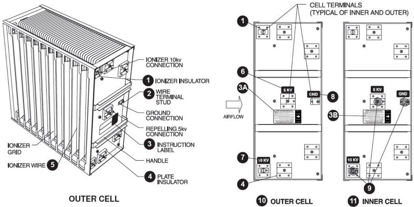
Figure 7-4-1 ESP Cells
