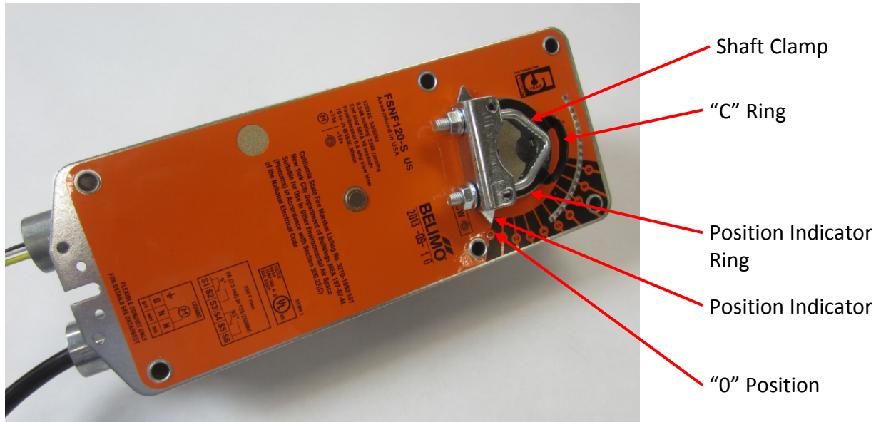
Figure 4-40-1 Oscillating Motor
