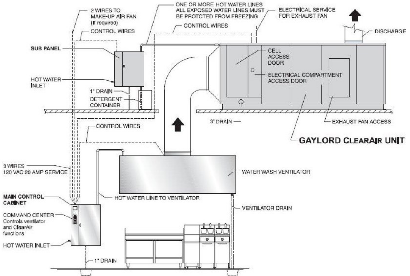
Figure 2-4-1 Typical Arrangement with Water Wash Ventilator with the Main Wash Control Cabinet Serving the Water Wash Ventilator and Sub Panel Serving the ClearAir Unit
