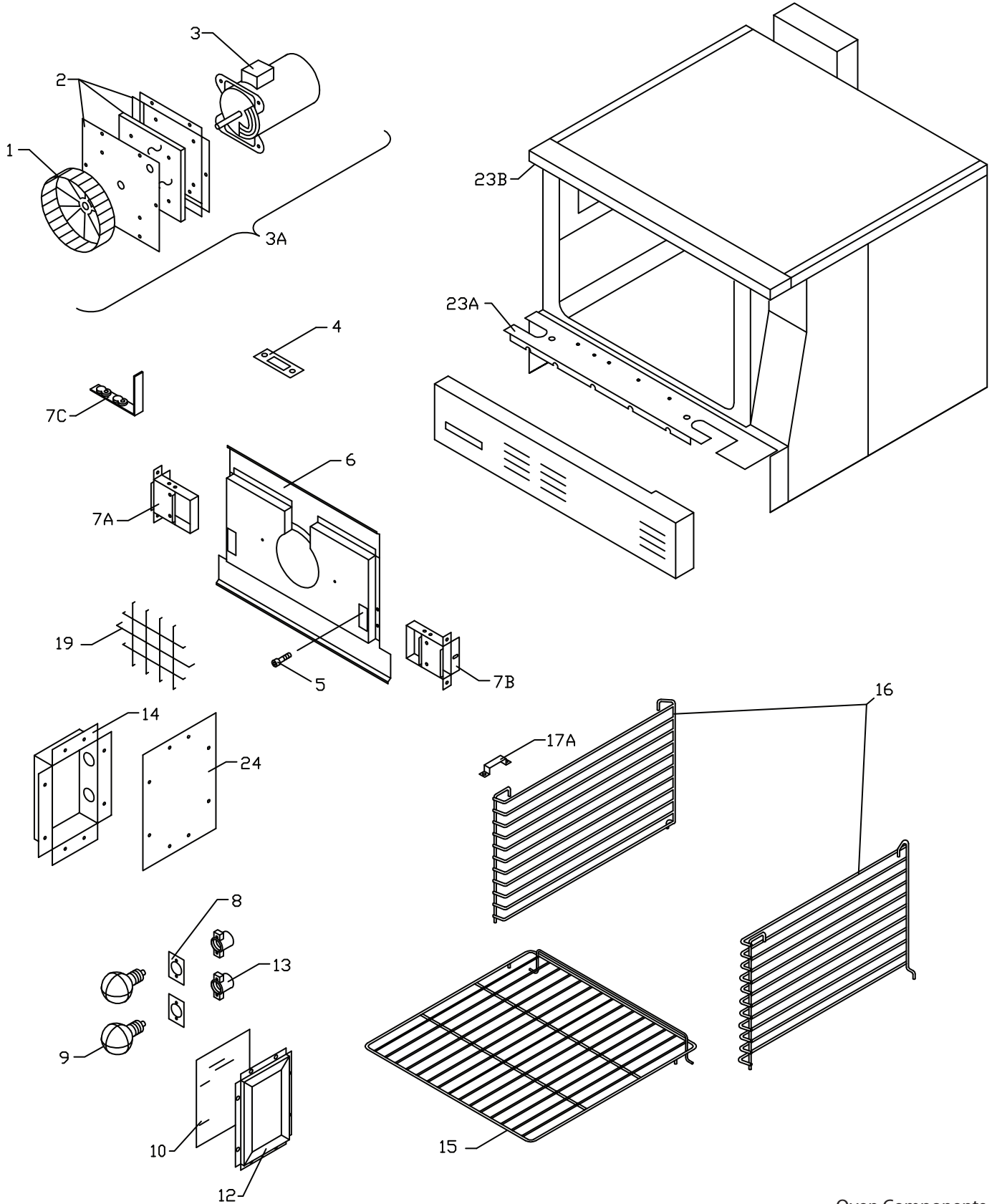
Oven Components
