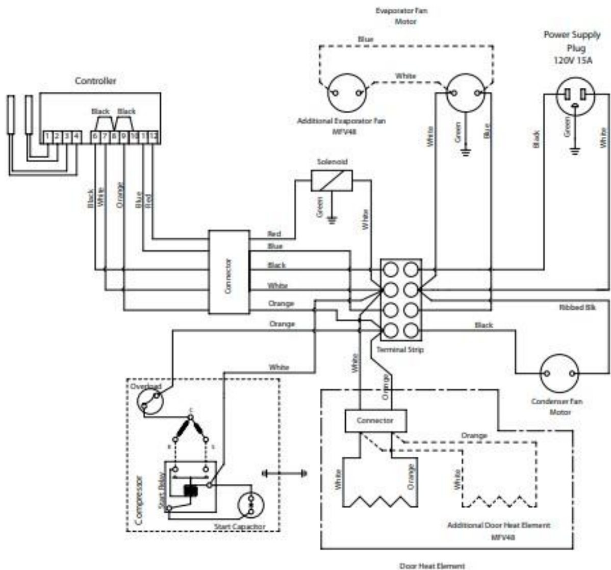
Evaporator/Condenser Unit
