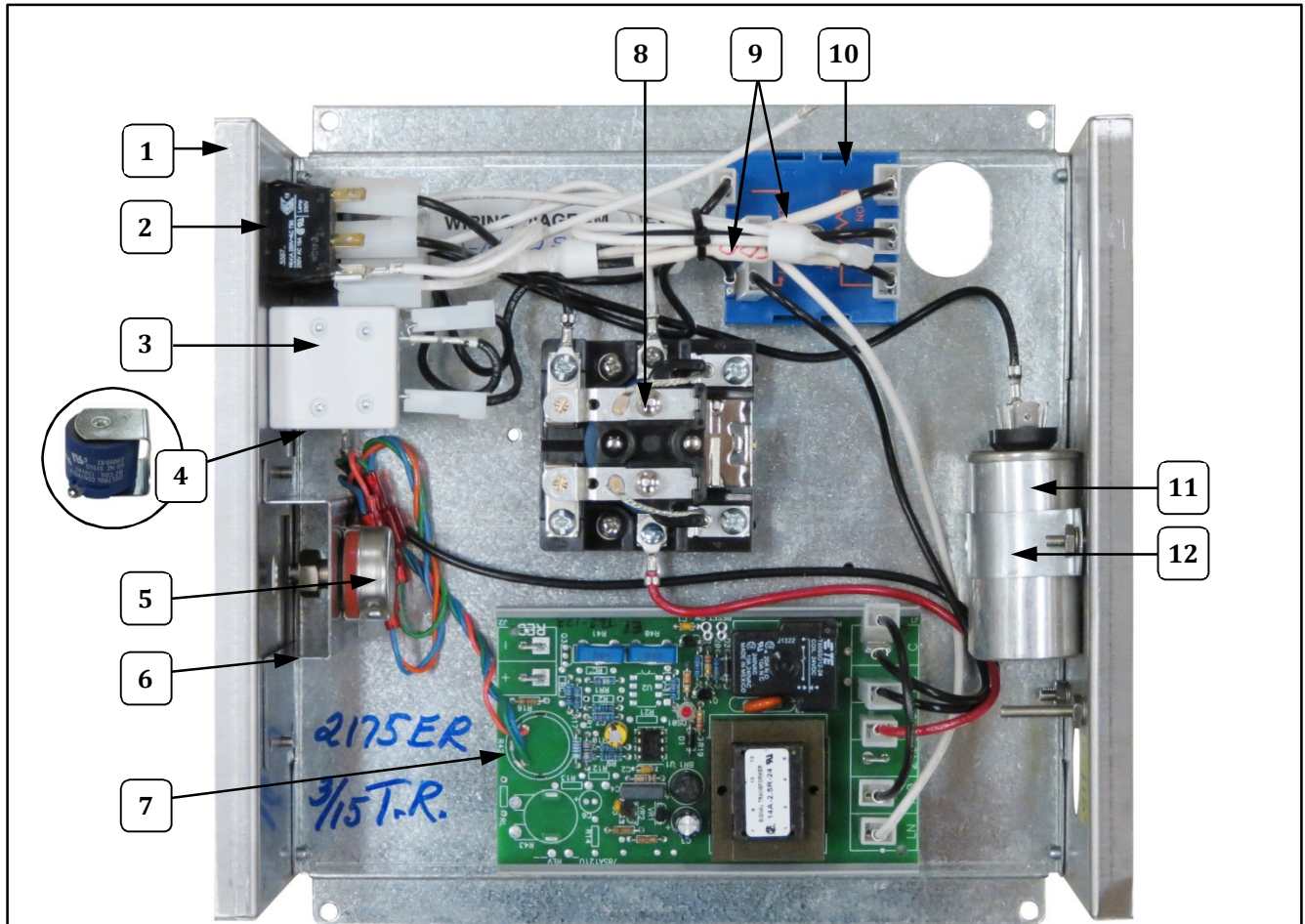
Control Panel Interior (Model 2175ER shown)
