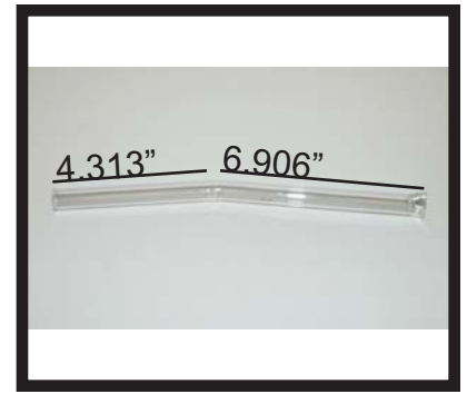
Spray Tube For 9 Liter Bowl
