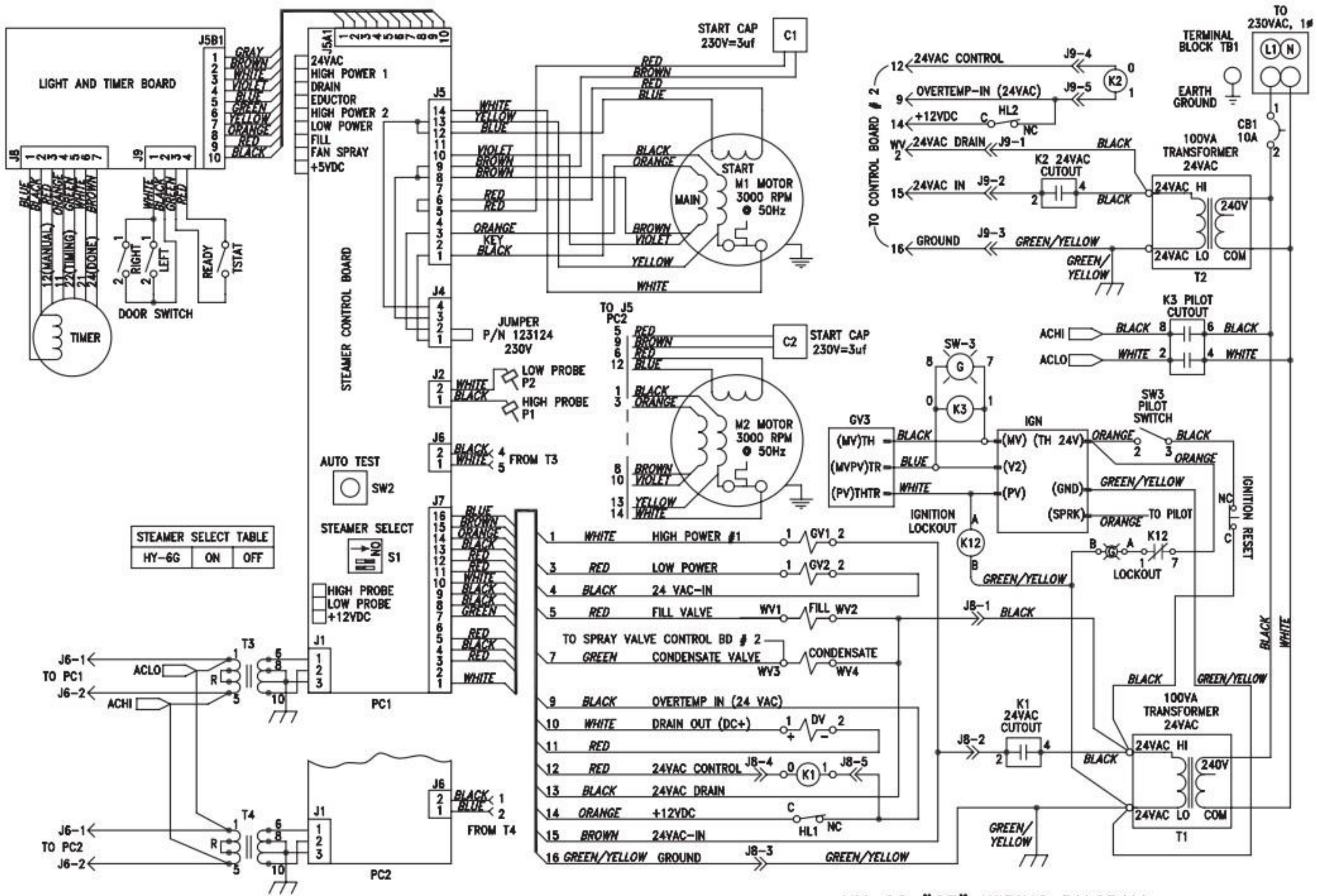
HY-6G "CE" WIRING DIAGRAM P/N 144149 REV C GROEN
