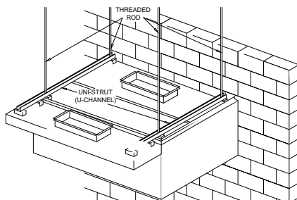
Air Curtain Supply (ASP) Mounted with uni-strut and threaded rod
