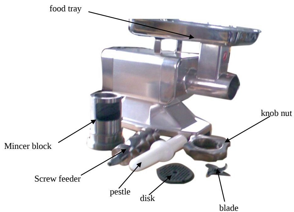
FIG 7-Diagram of GSM-50 and GSM-100 stripped for cleaning
