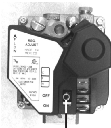
Gas Control Valve “ON/OFF” Selector
