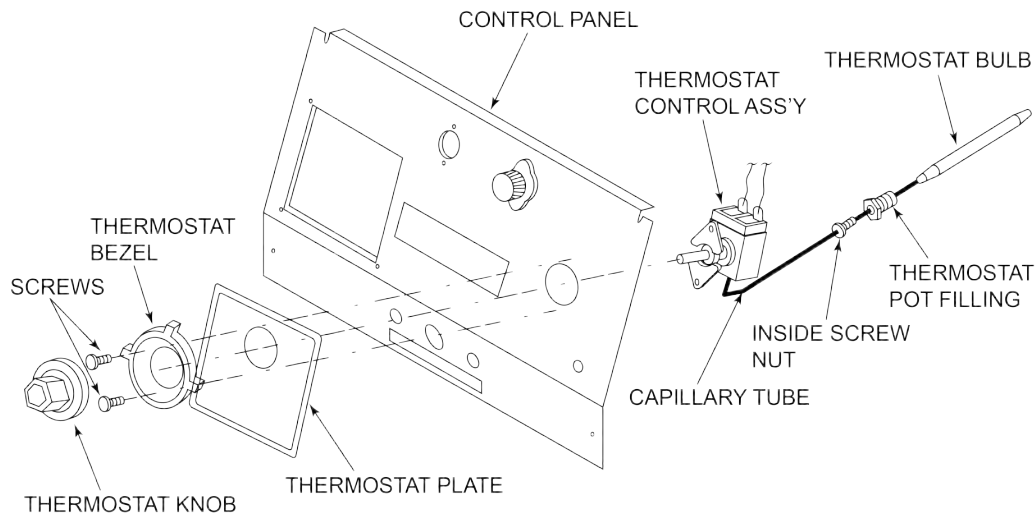
Figure 2-3 Thermostat & Control Panel Diagram
