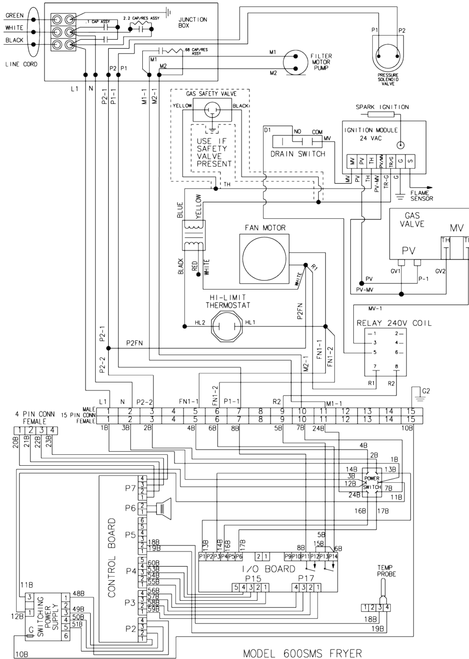
MODEL 600SMS FRYER 230V 50HZ 1PH SMS SSI CONTROL HENNY PENNY CORP., EATON, OHIO 45320 75512
