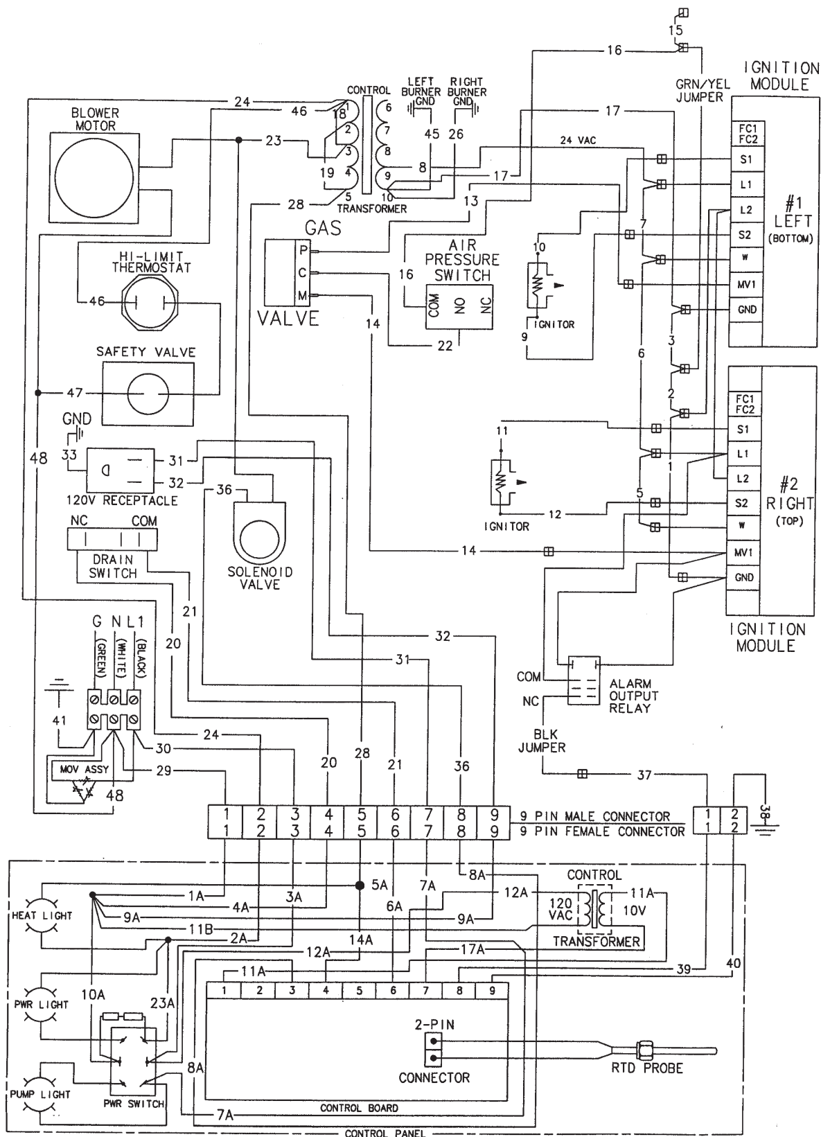
8-HEAD GAS COOKER W/LOCAL FLAME SENSING 120V 1PH 2W + G 54789
