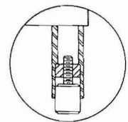
ENLARGED VIEW OF LEG SHOWING ADJUSTING FOOT
