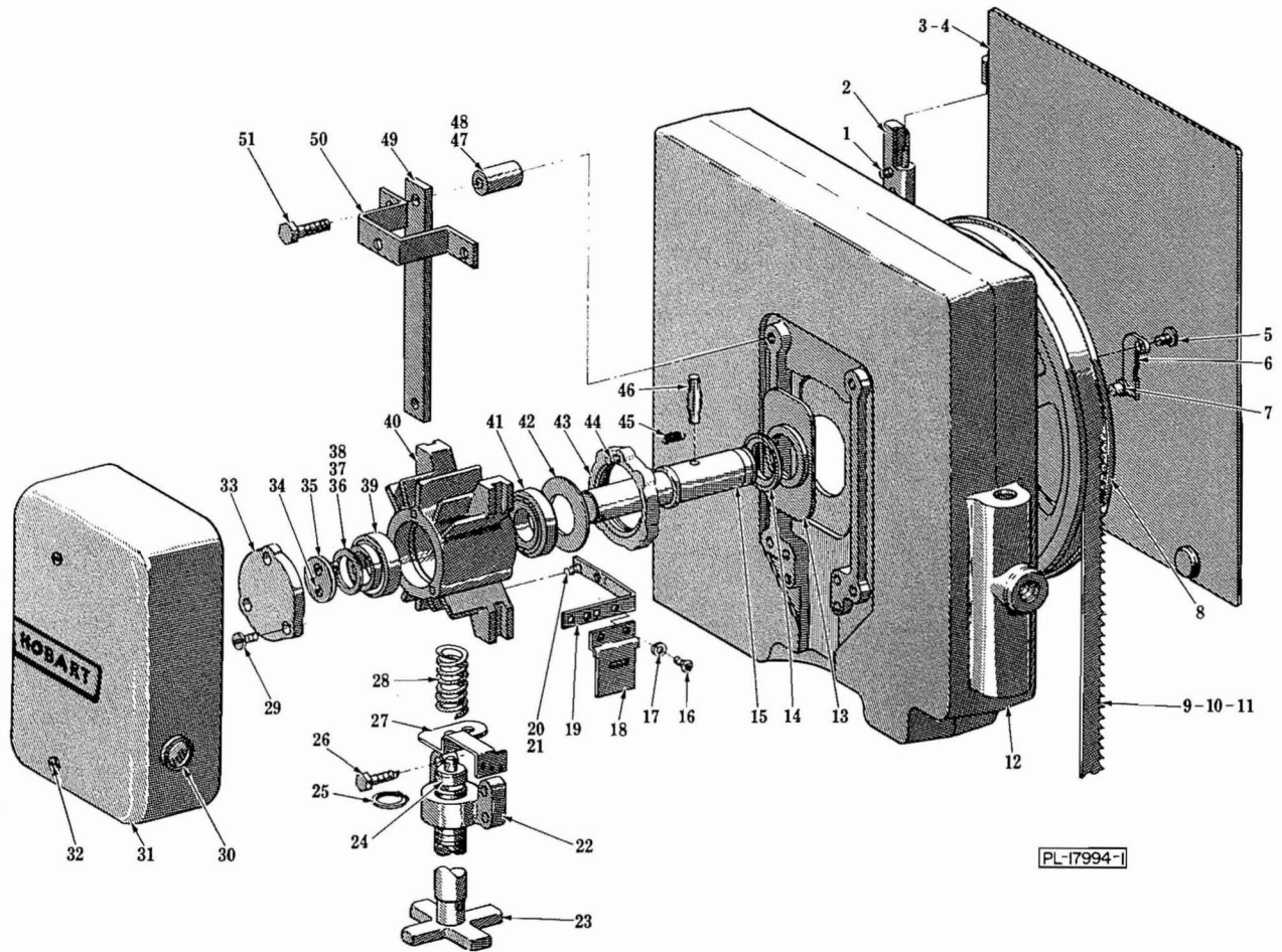
HEAD UNIT
