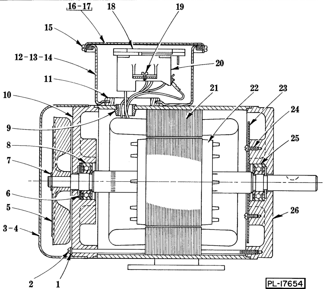
MOTOR UNIT
