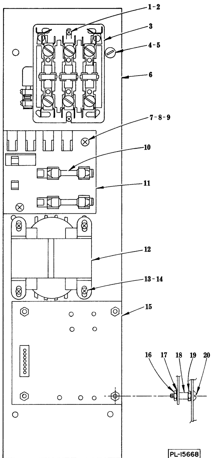
CONTROL PANEL (BLOWER DRYER)
