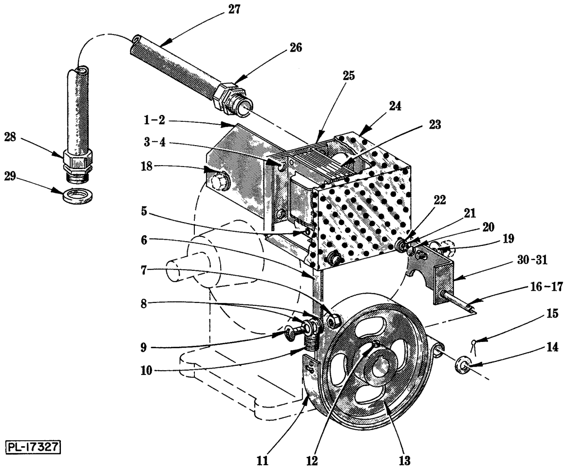
CONVEYOR BRAKE
