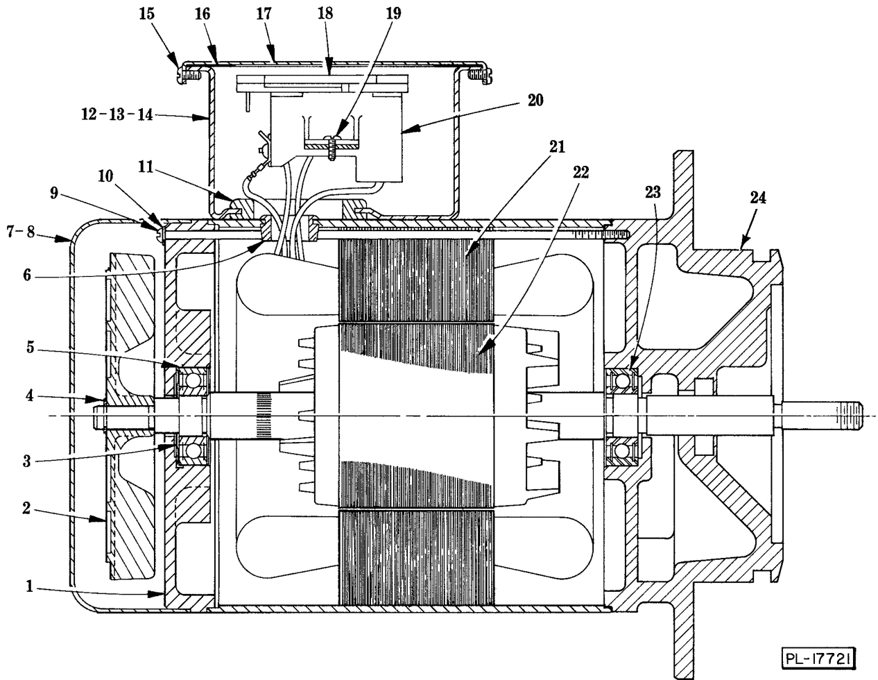
MOTOR UNIT
