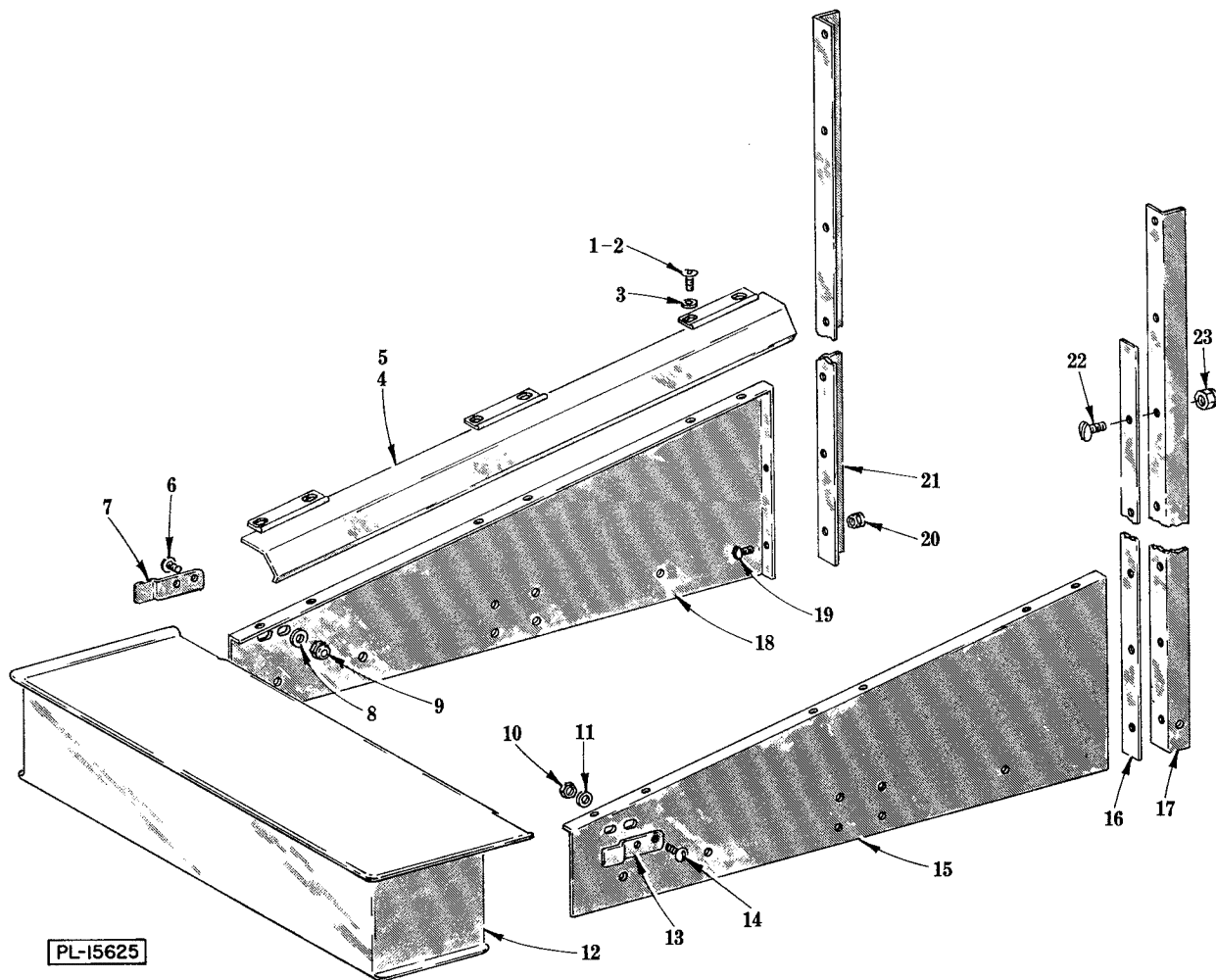
DISH PLATFORM AND EXTENSION PANELS (WITH BLOWER DRYER)
