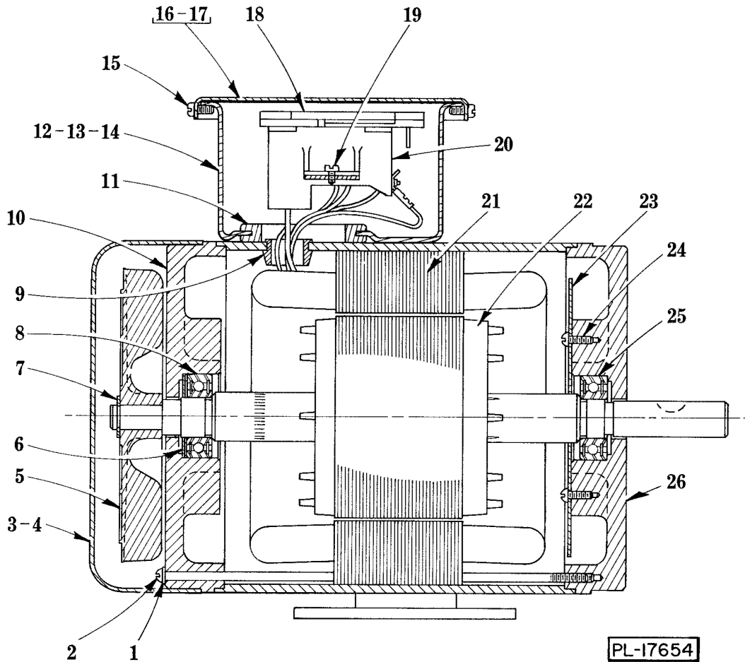
MOTOR UNIT
