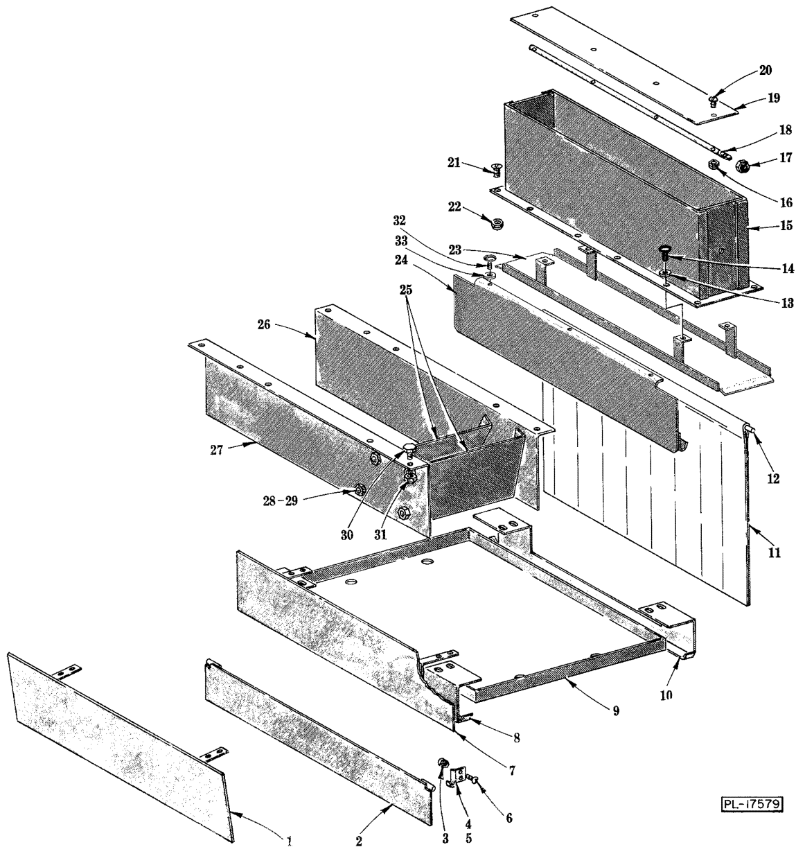
BLOWER BAFFLES AND VENT
