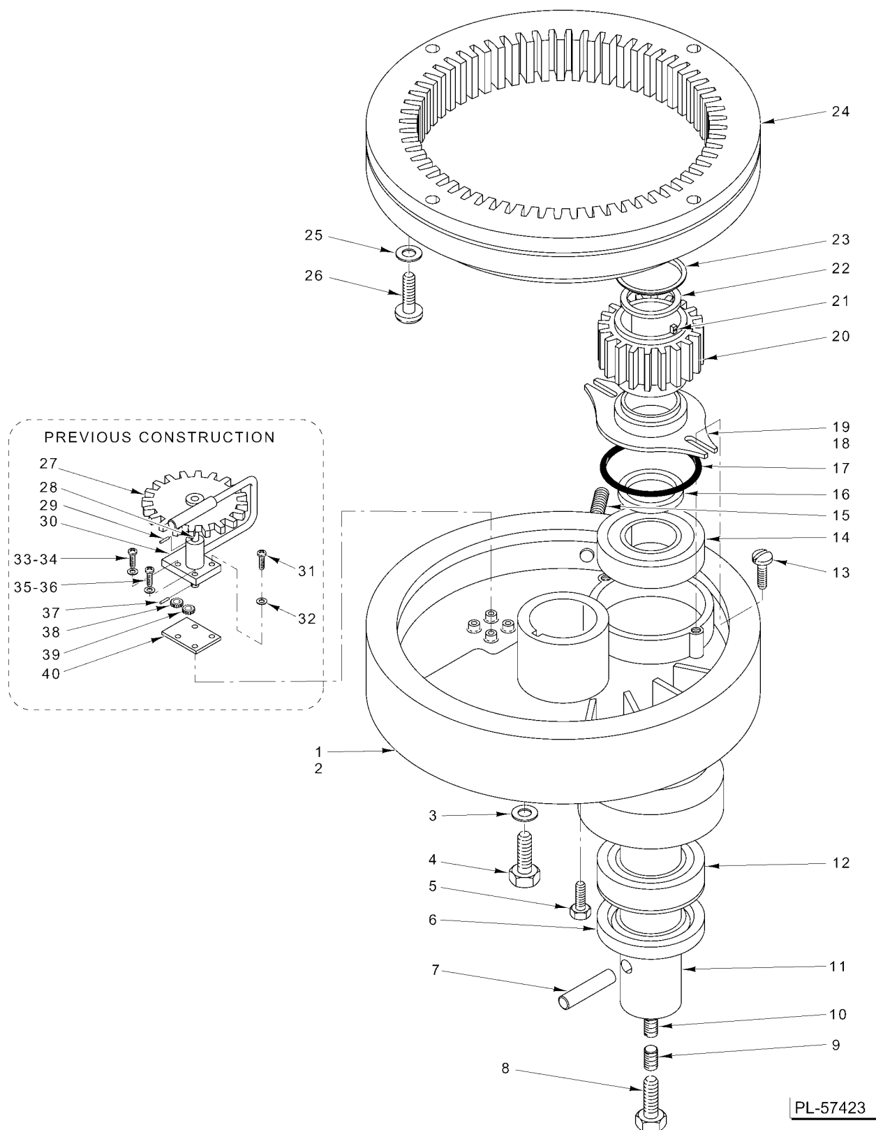
PLANETARY UNIT
