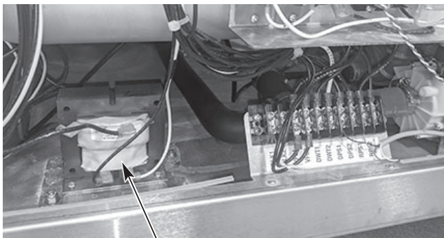
1T TRANSFORMER (PW20/PW20eR LOCATION SHOWN)
