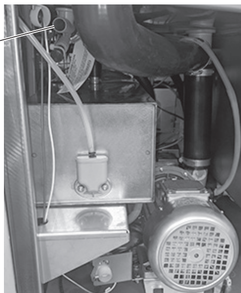
CONNECT DRAIN HOSE AT BARBED FITTING (VIEW FROM BACK OF MACHINE)
