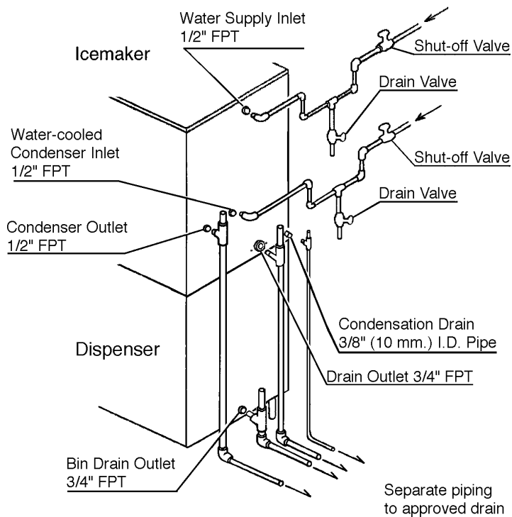
Fig. 4 Drain Connection
