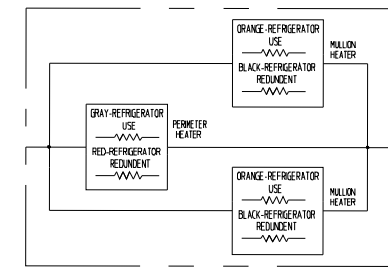
PERIMETER HEATER WIRING (HEATERS WIRED IN PARALLEL) (MULLION HEATER QUANTITY 1 PER MULLION) (RH3 SHOWN)
