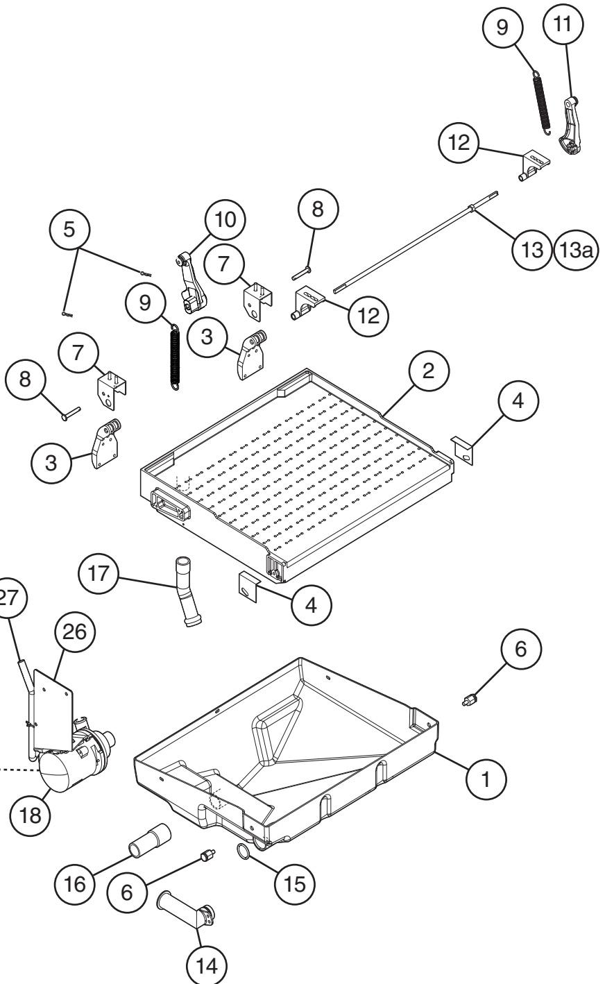
Mechanism Assembly
