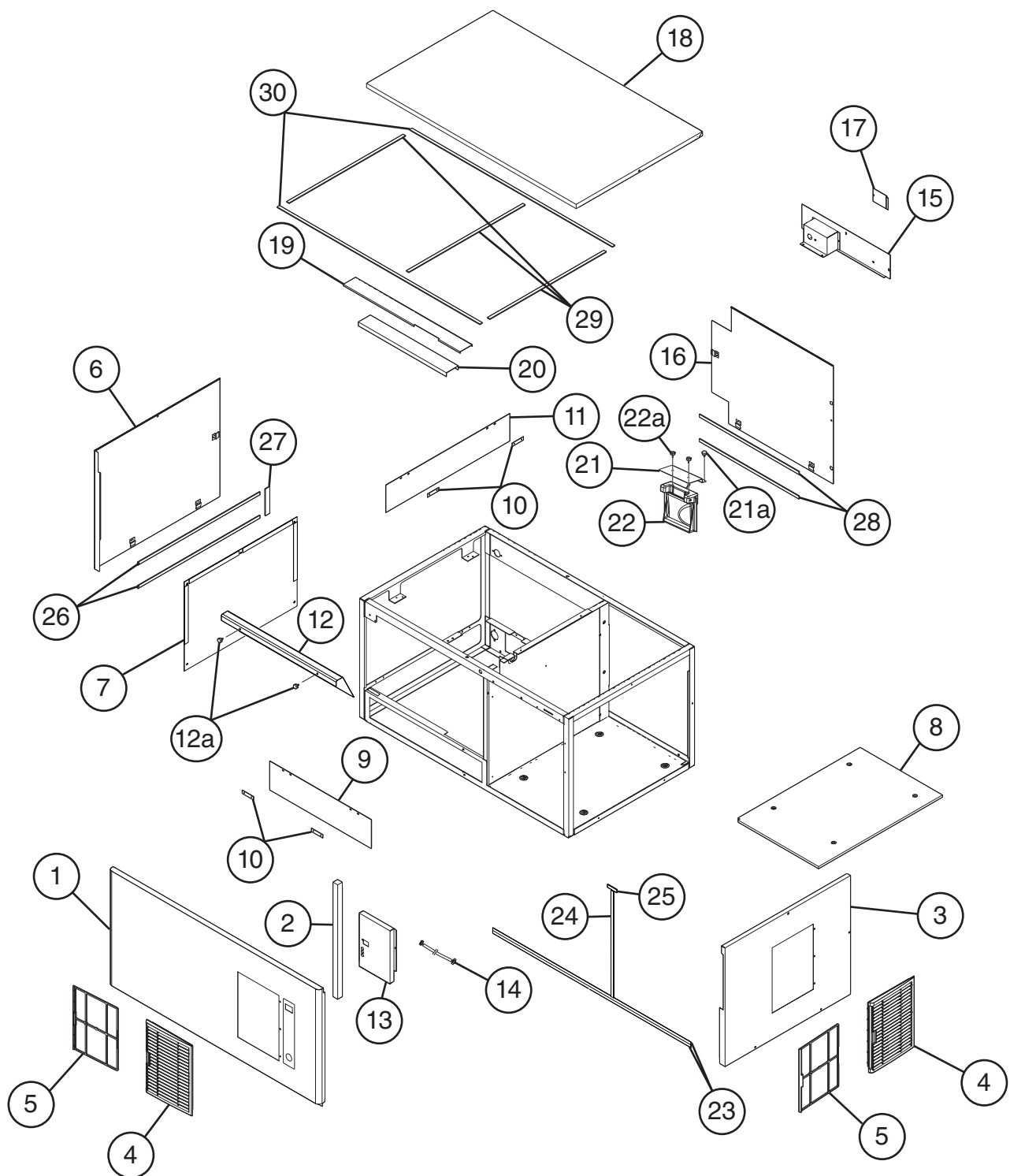
Main Assembly
