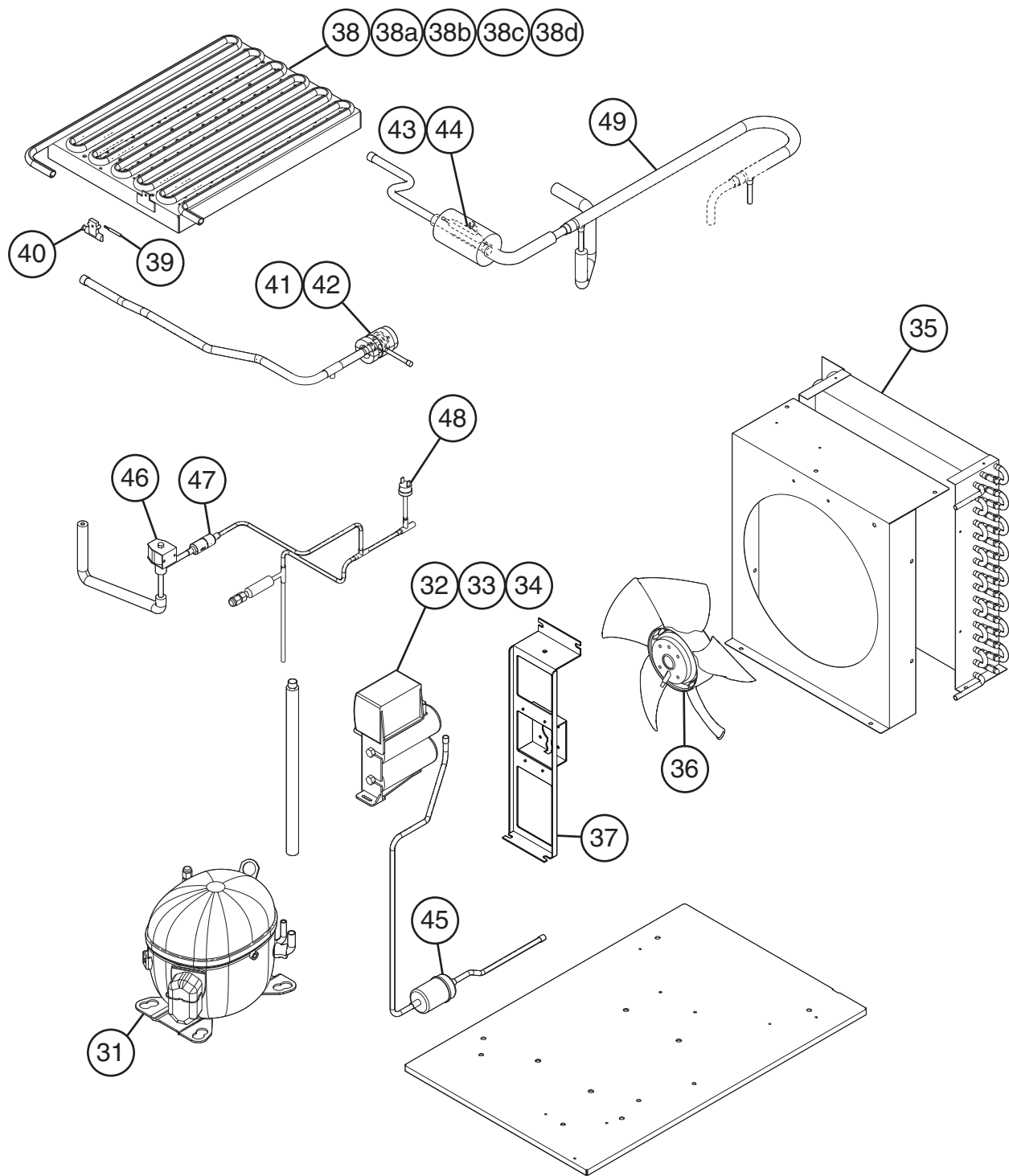
Refrigeration Circuit
