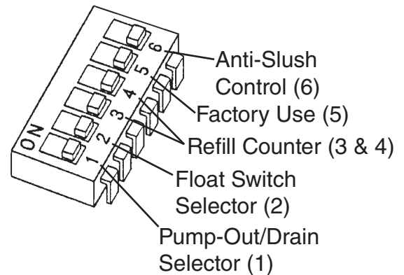
S2 Dip Switch
